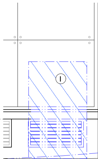
4 Elevation AA - Localised Scale: 1:50
