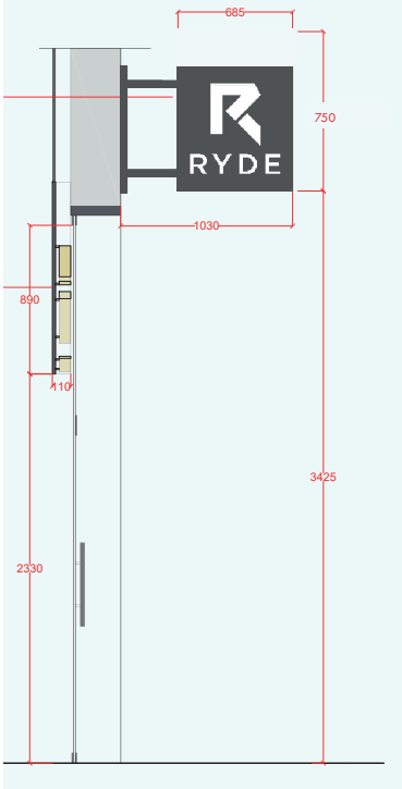
SECTION
