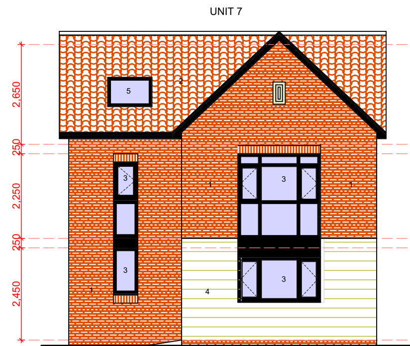
PROPOSED GA FRONT ELEVATION UNIT 7
