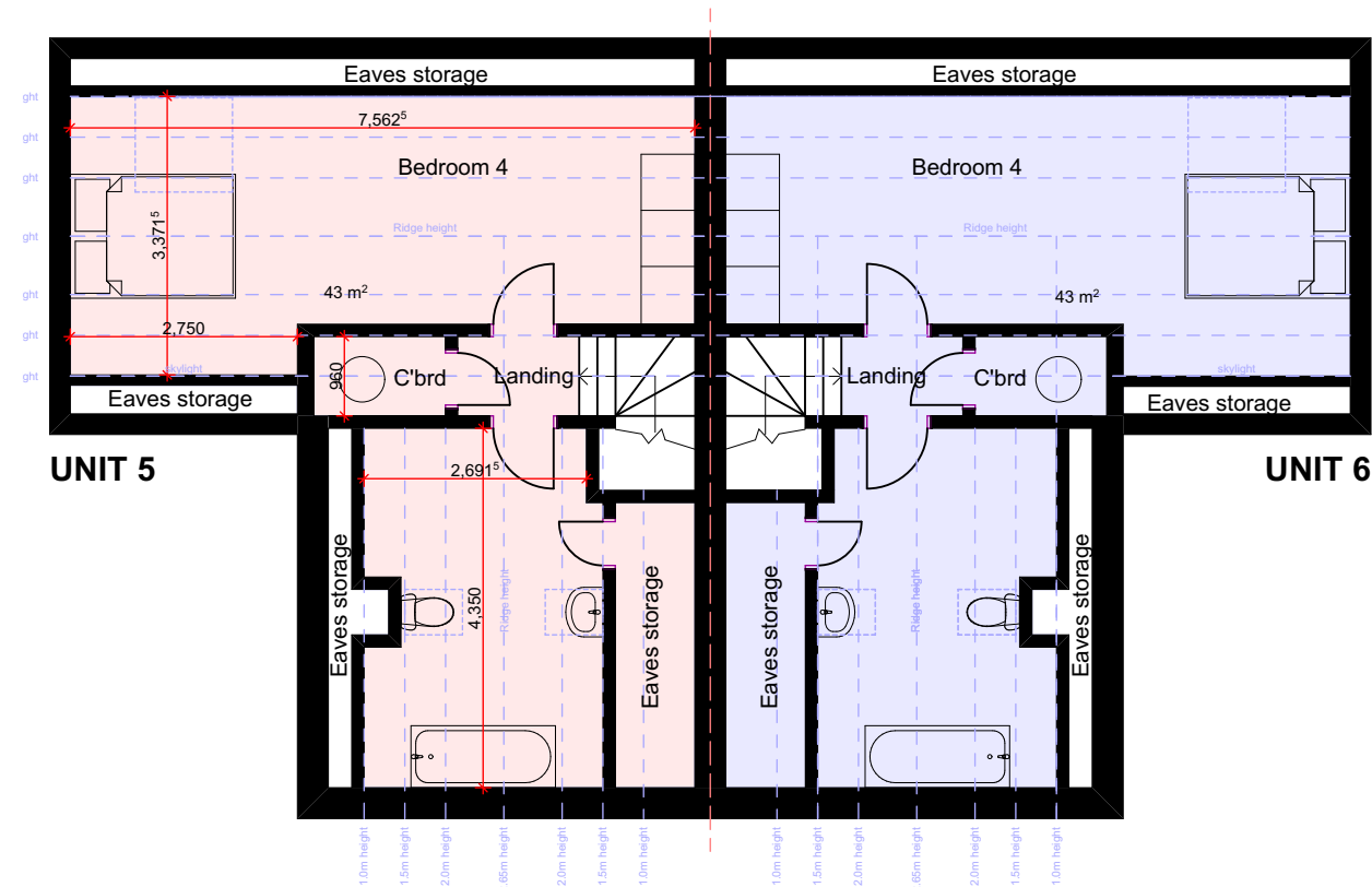
PROPOSED GA SECOND FLOOR PLAN
