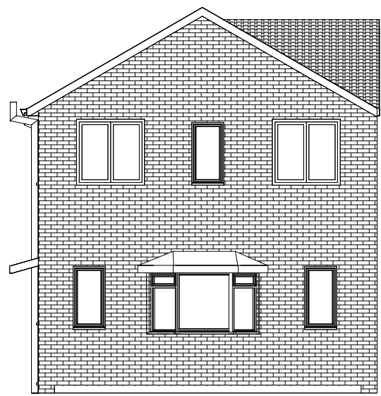
Existing Front 1 : 100
