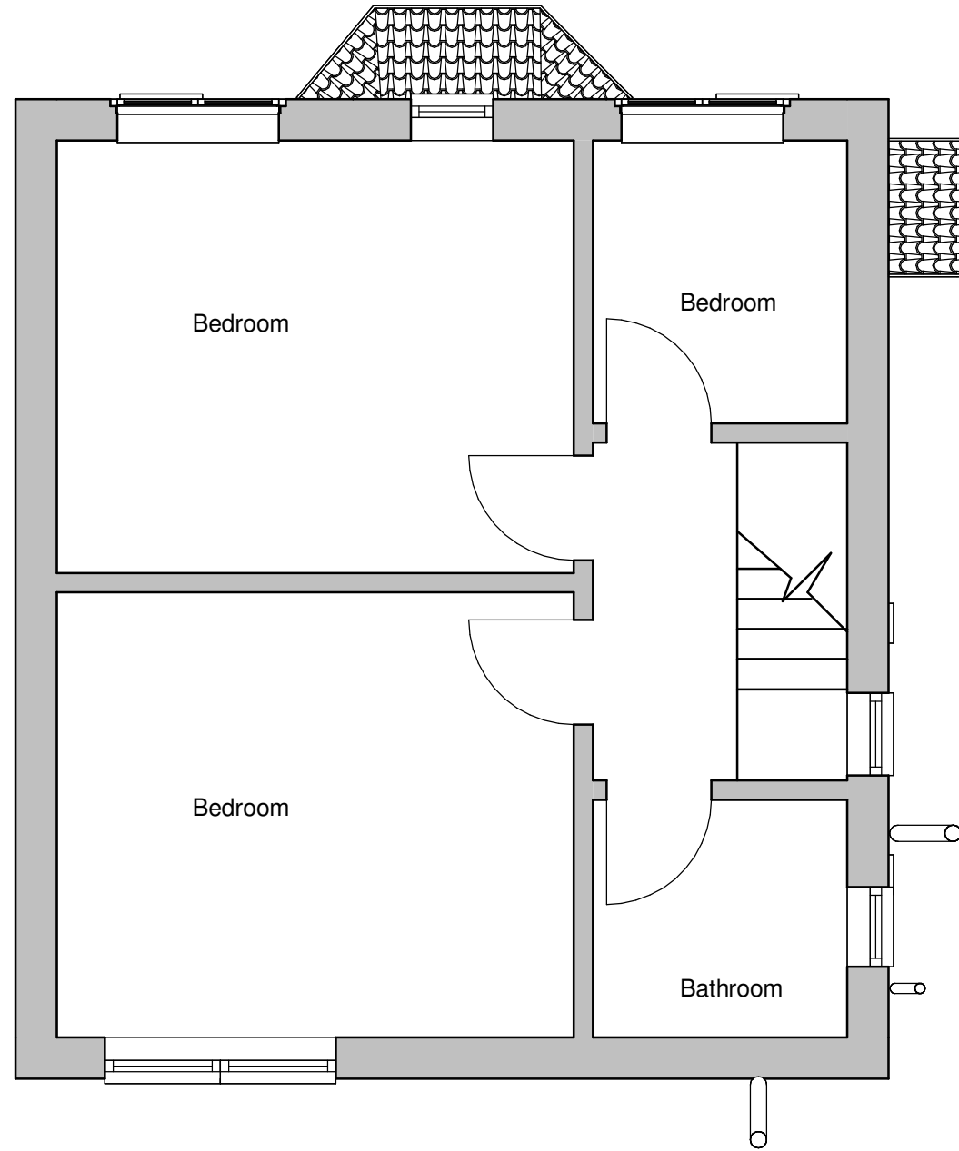
Existing First Floor 1 : 50
