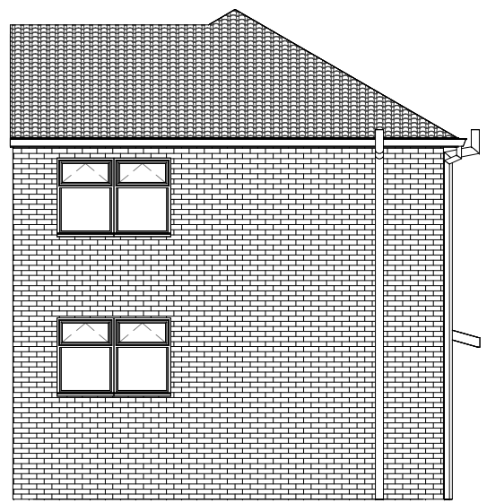
Existing Rear 1 : 100
