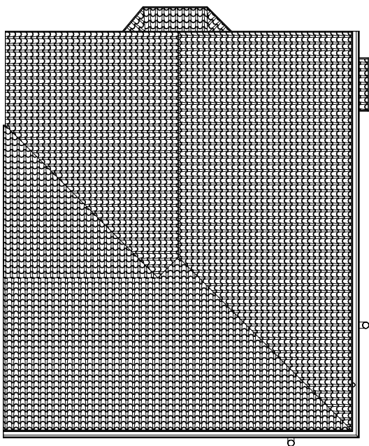
Existing Roof Plan 1 : 100
