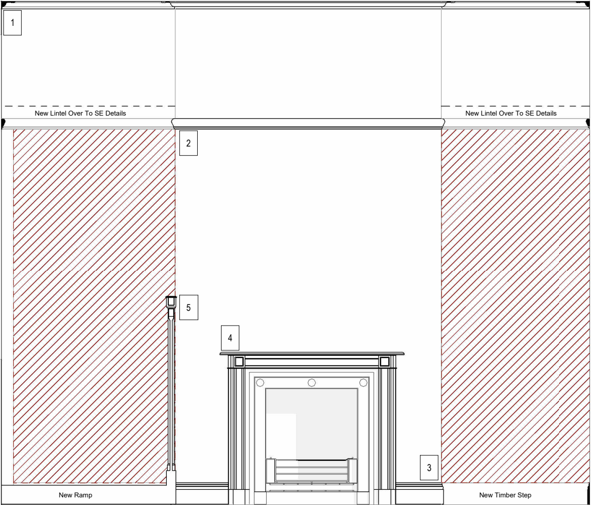
2 Intervention Elevation - Typical Fireplace
