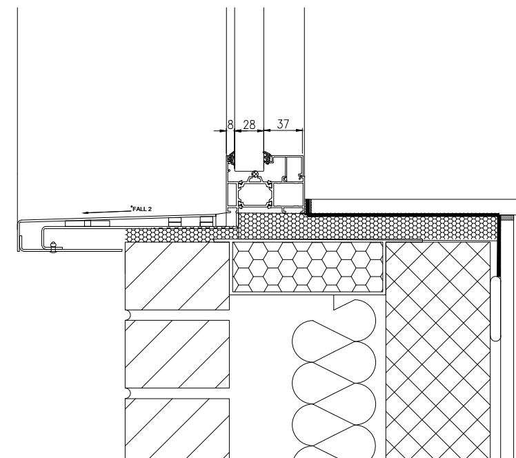
Section Profile 1:5 @ A3
