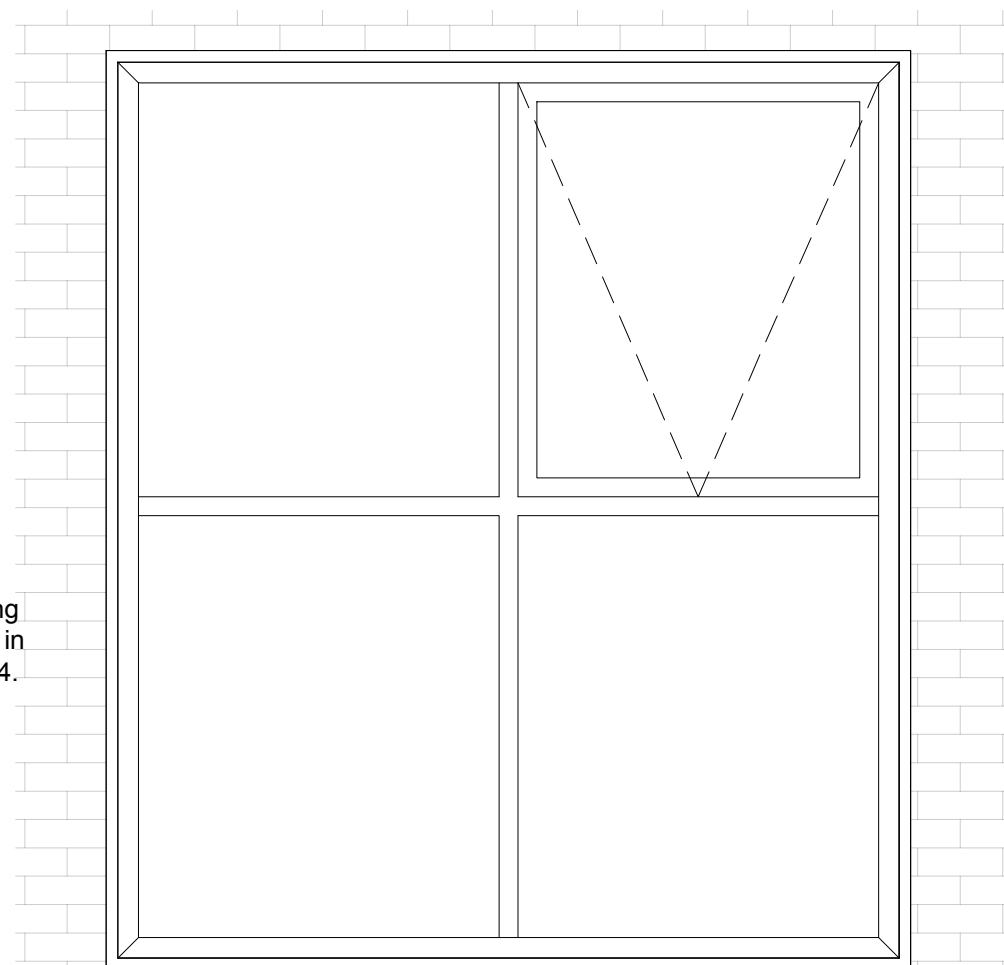
Window Elevation 1:20 @ A3
