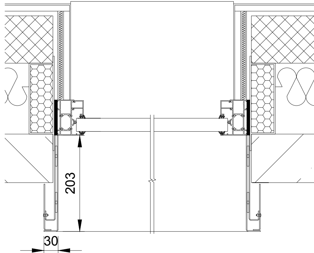
Window Plan 1:5 @ A3
