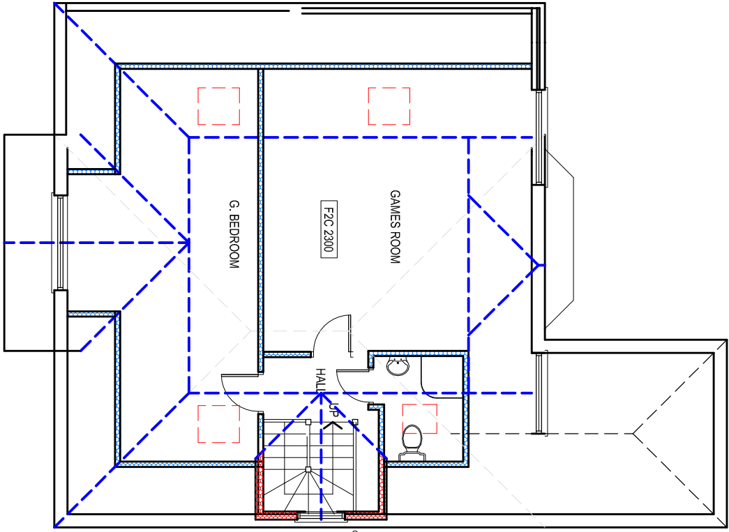
PROPOSED LOFT PLAN
