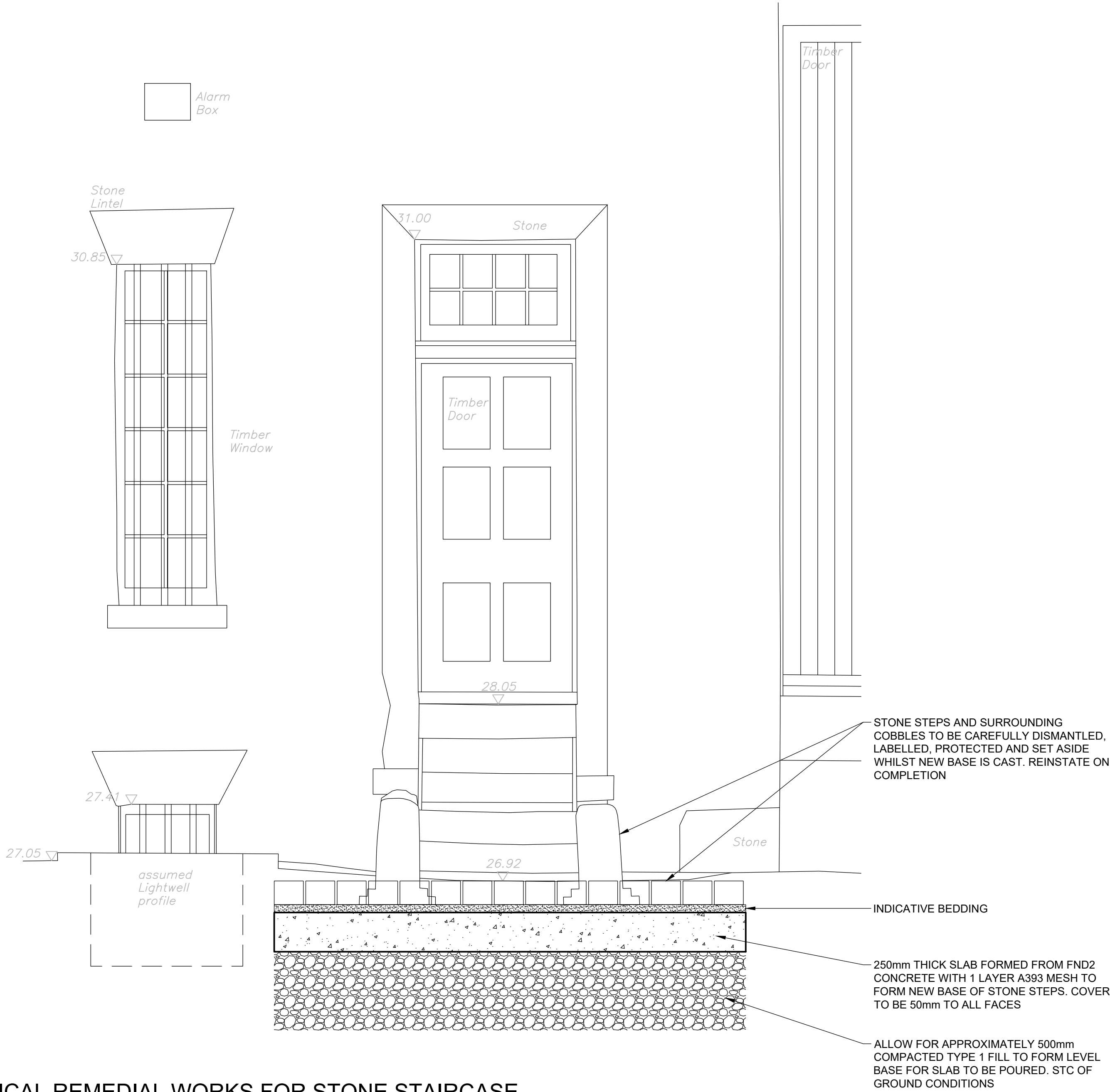
7 TYPICAL REMEDIAL WORKS FOR STONE STAIRCASE 1:20
