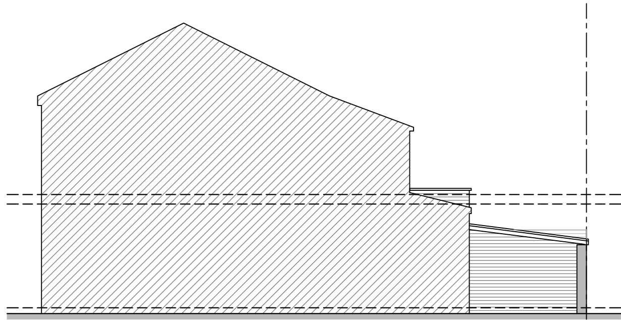
RIGHT ELEVATION 1:100
