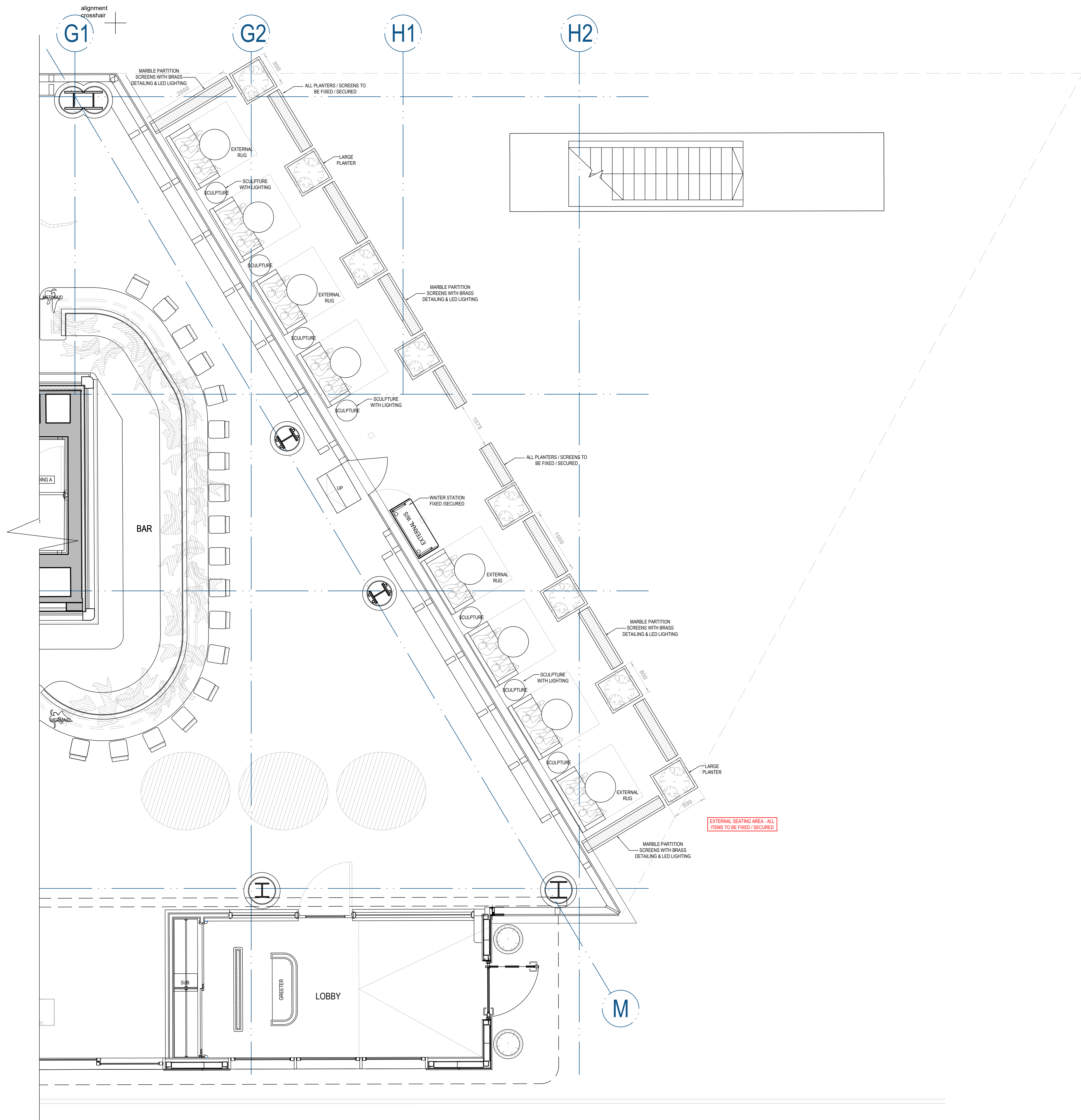
PROPOSED EXTERNAL SEATING PLAN
