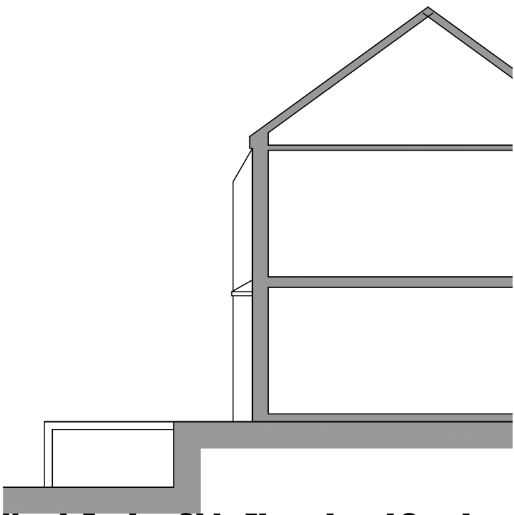
North Facing Side Elevational Section
