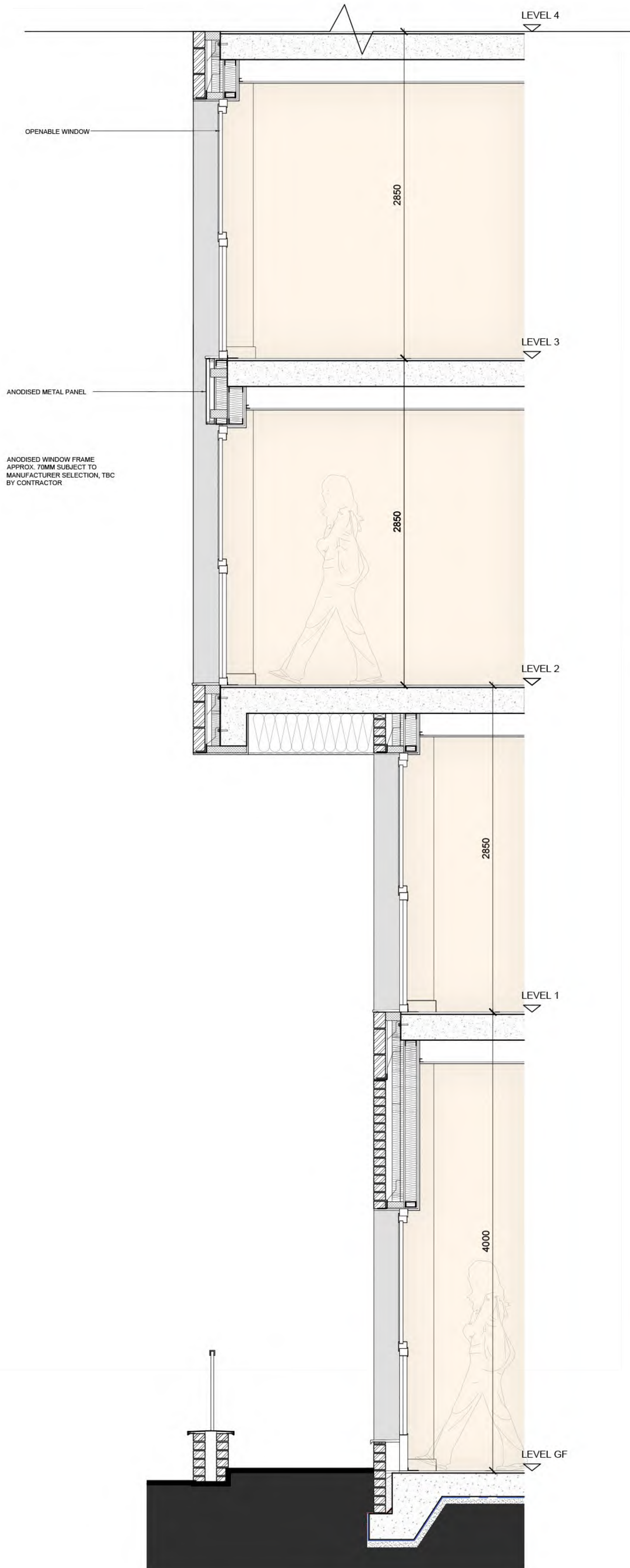
EXTERNAL WALL DETAIL SECTION A-2
