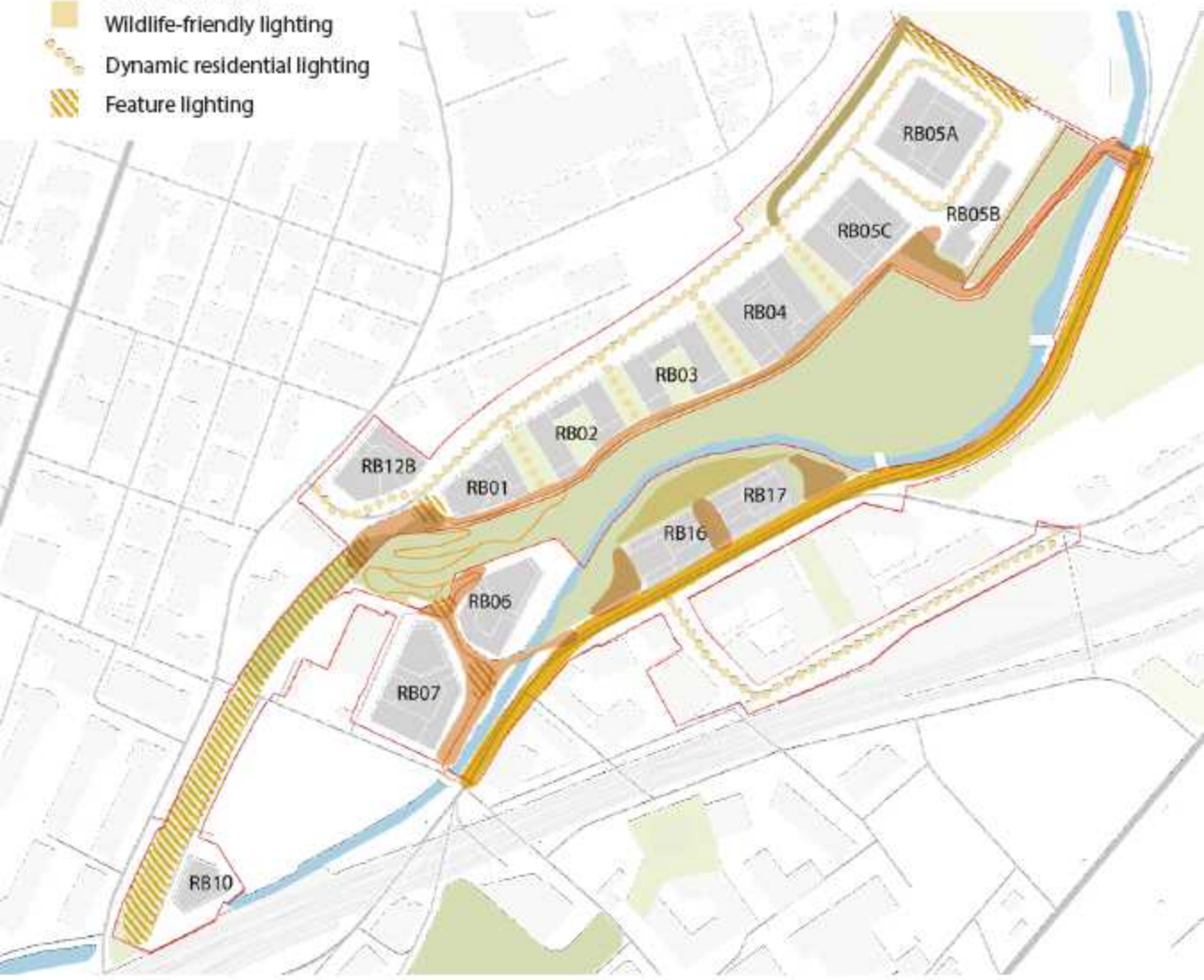
Dynamic LED Street Lighting
