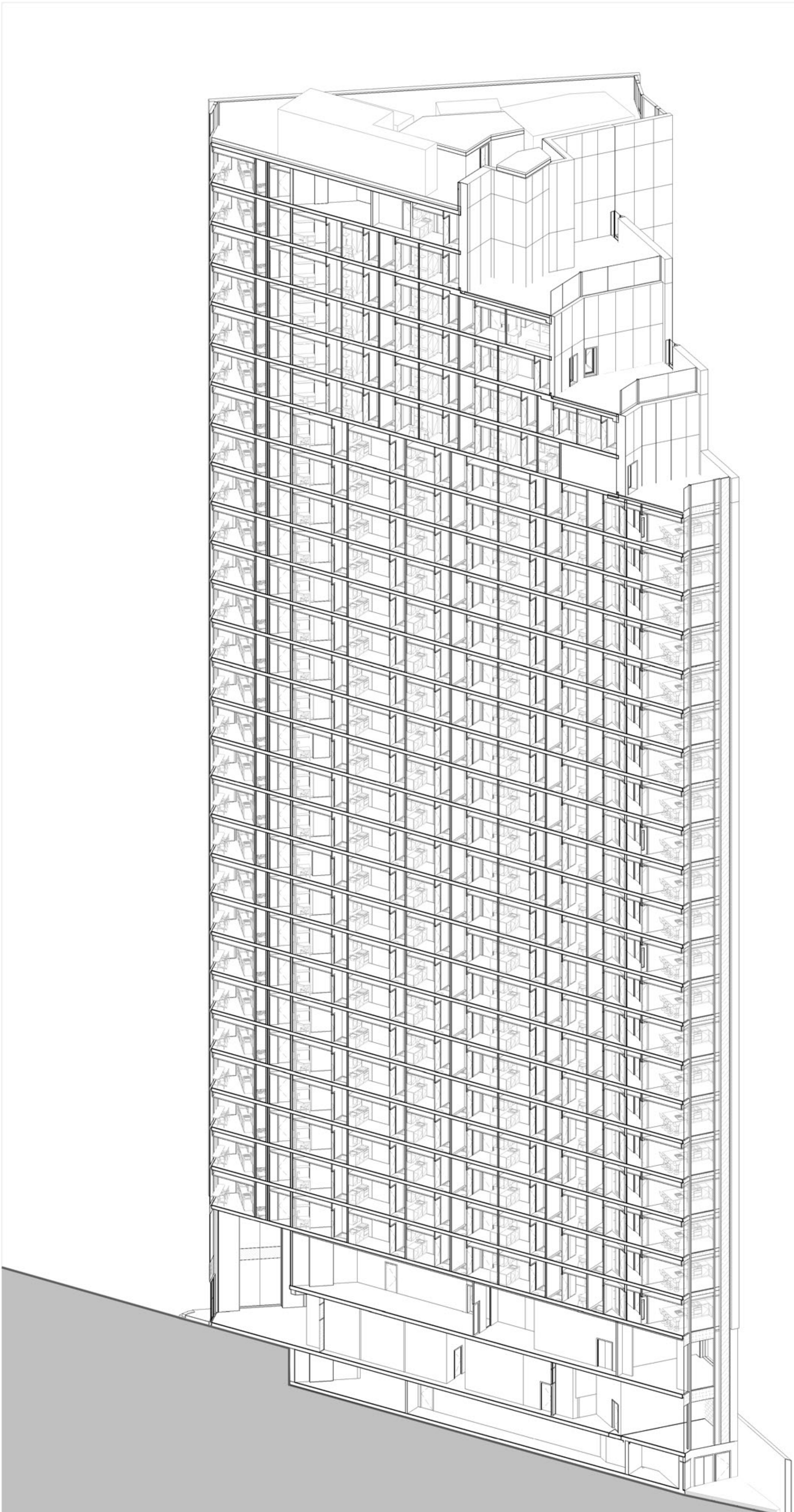
02 1:200 - 3D Isometric Section - A-A
