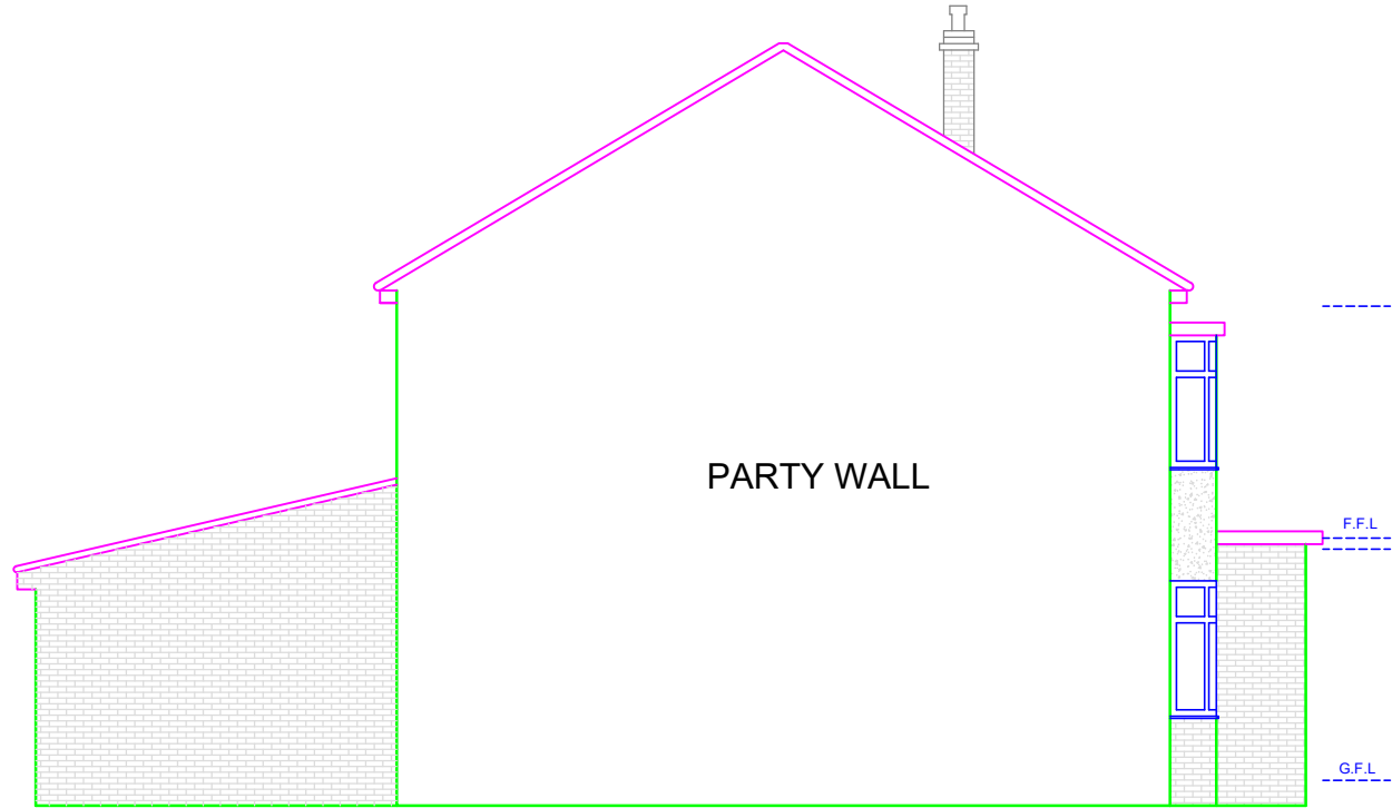
PROPOSED SIDE ELEVATION (NORTH)
