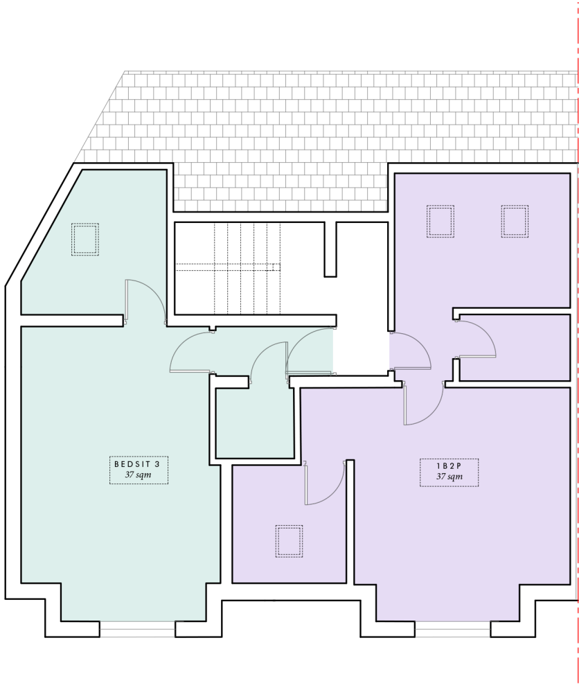
EXISTING SECOND FLOOR 1:100 @ A3 NO CHANGES
