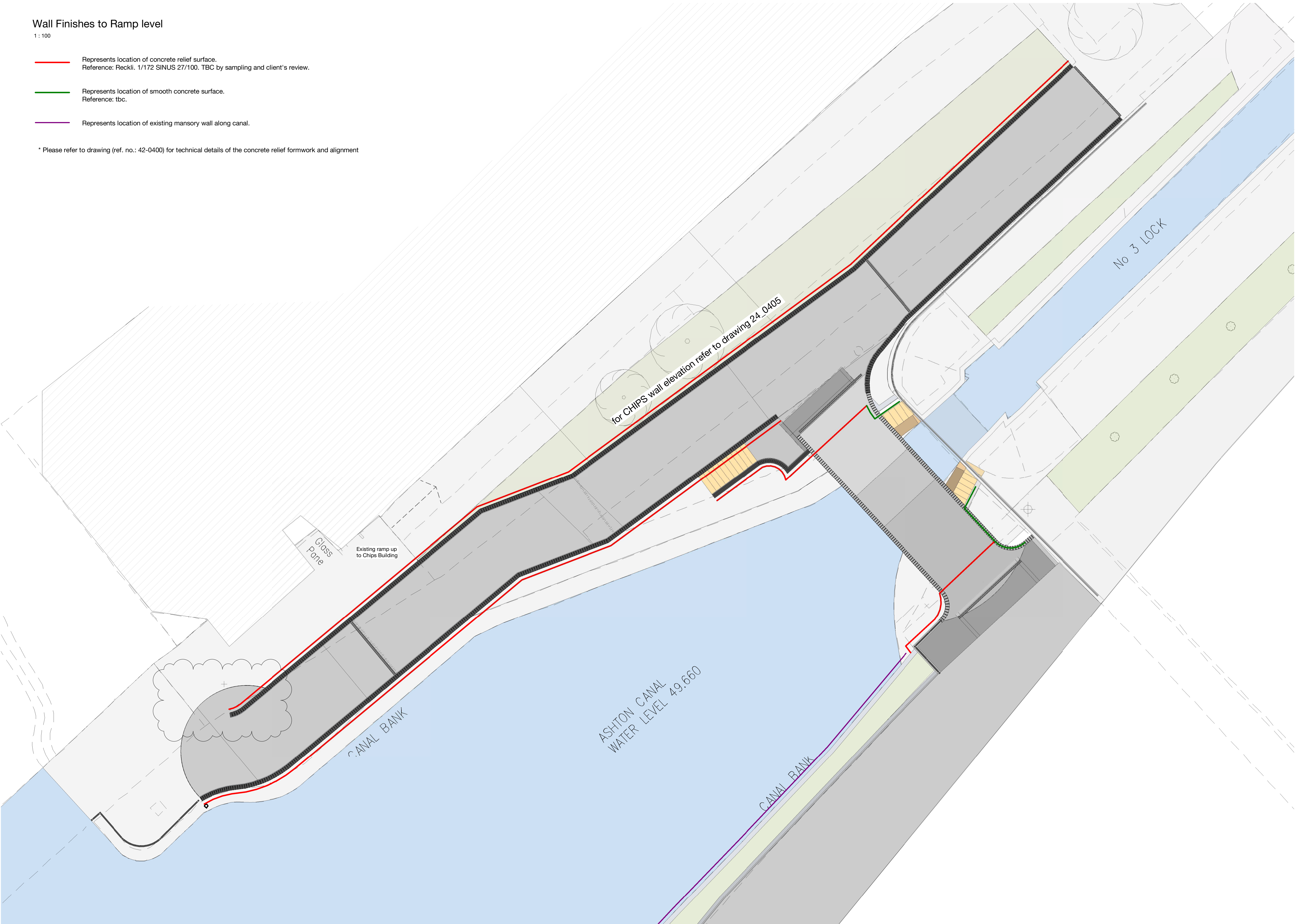
1 Ramp and Bridge Concrete Relief Extent 1 : 100
