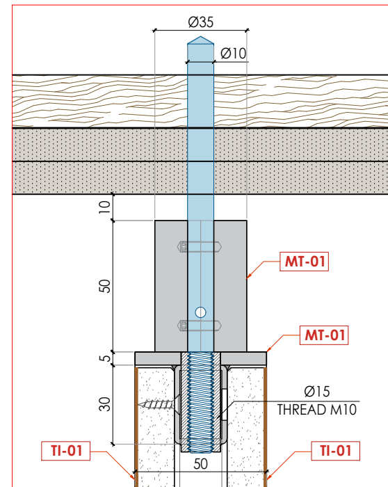
Detail 1 Scale 1:2
