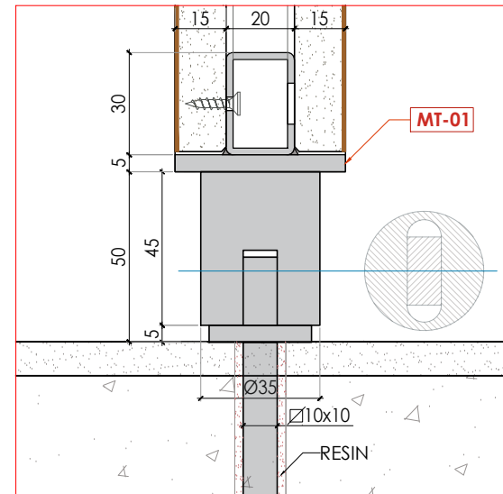
Detail 2 Scale 1:2
