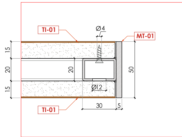
Detail 3 Scale 1:2
