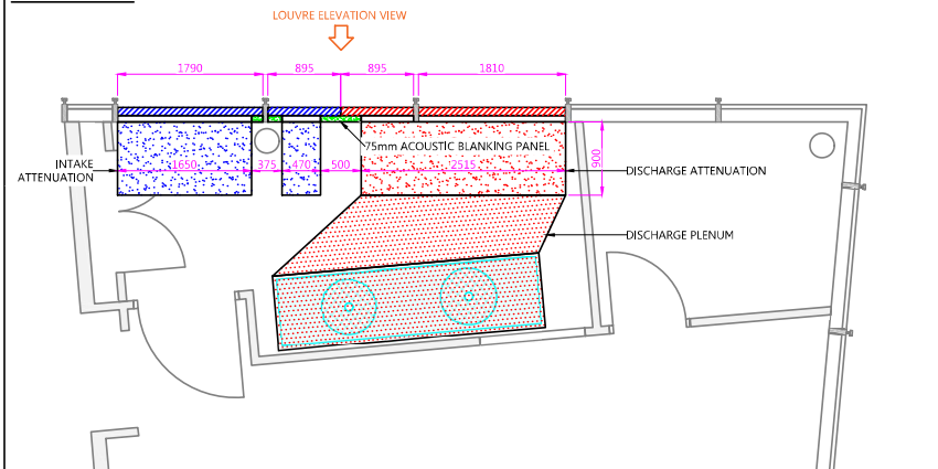
HIGH LEVEL PLAN VIEW
