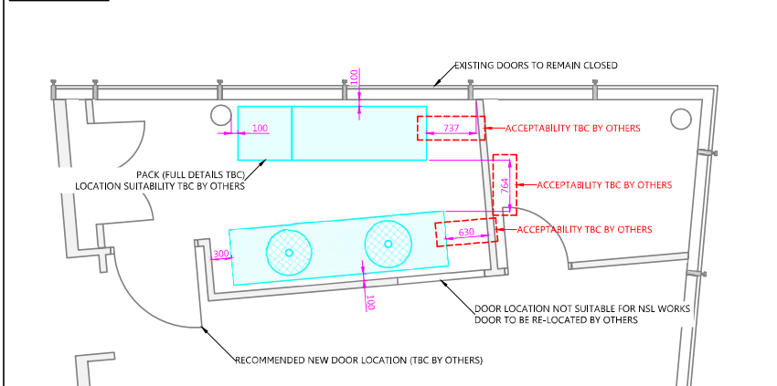
LOW LEVEL PLAN VIEW
