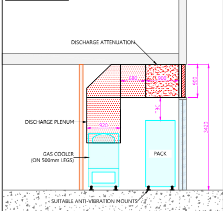
INDICATIVE SECTION VIEW
