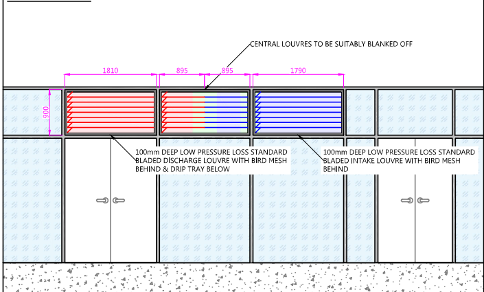
LOUVRE ELEVATION VIEW
