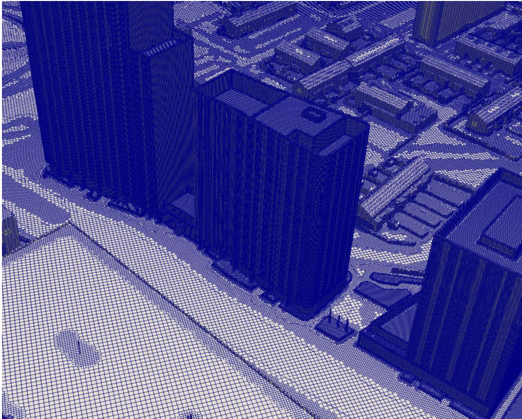
Figure A11.1 Mesh Detail on Site Buildings
