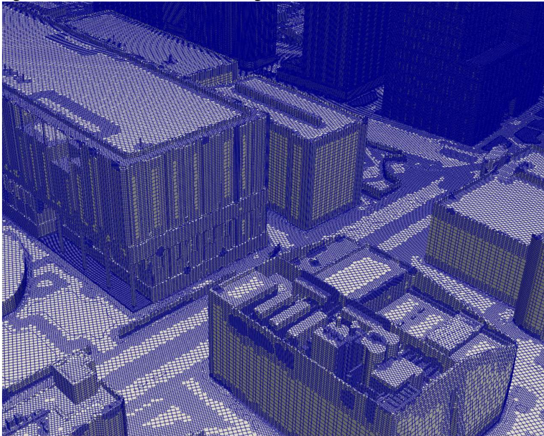
Figure A11.1 Mesh Detail on Site Buildings
