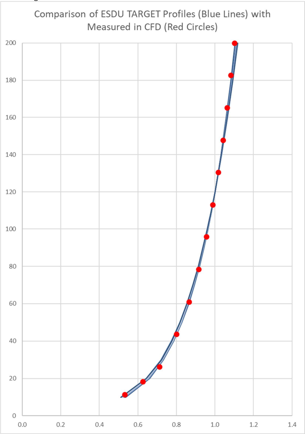
Figure A11.4 Wind Profile for Upper Brook Street
