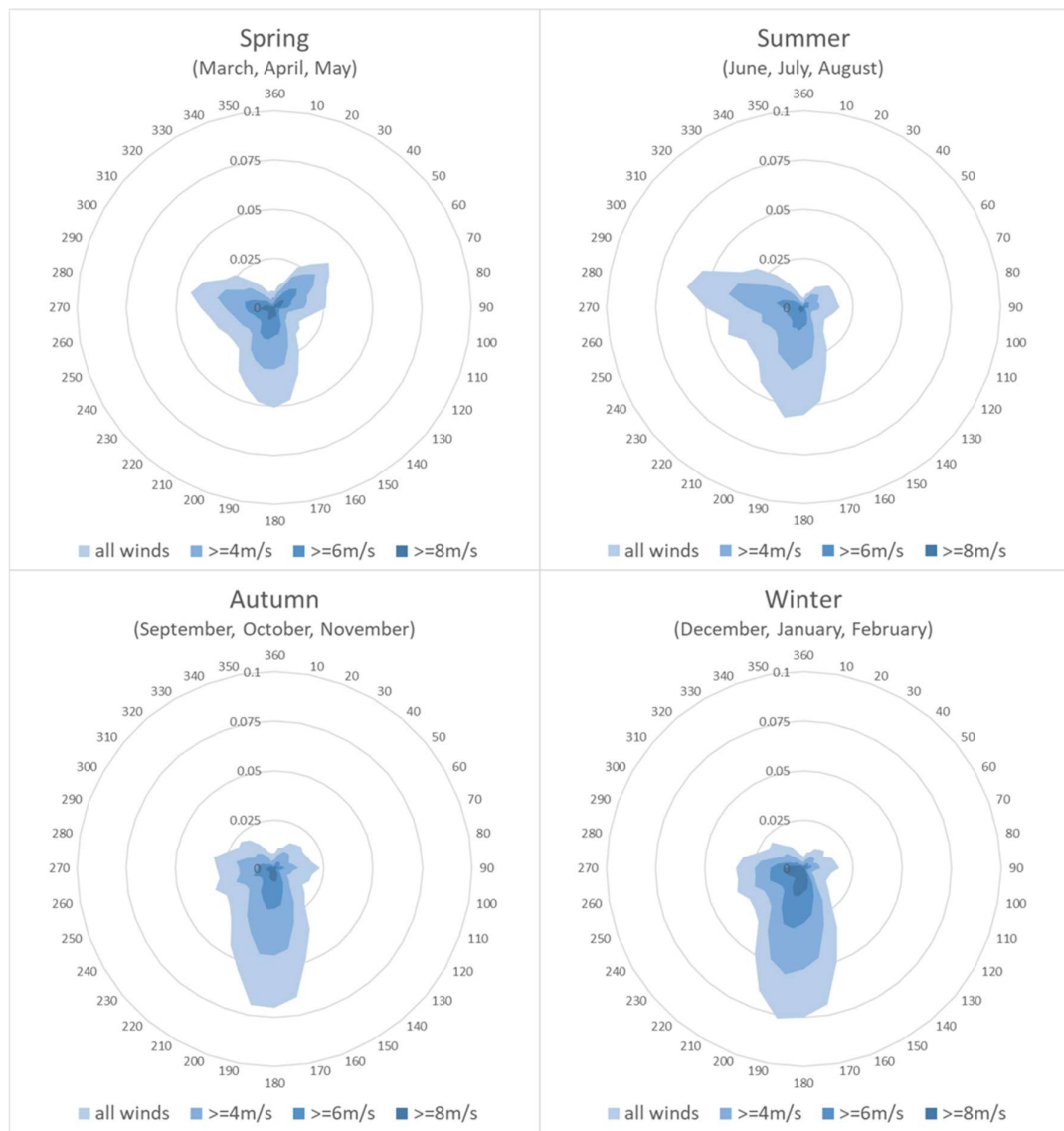
Figure A11.3 Seasonal Wind Roses for Manchester International Airport (1990-2020)
