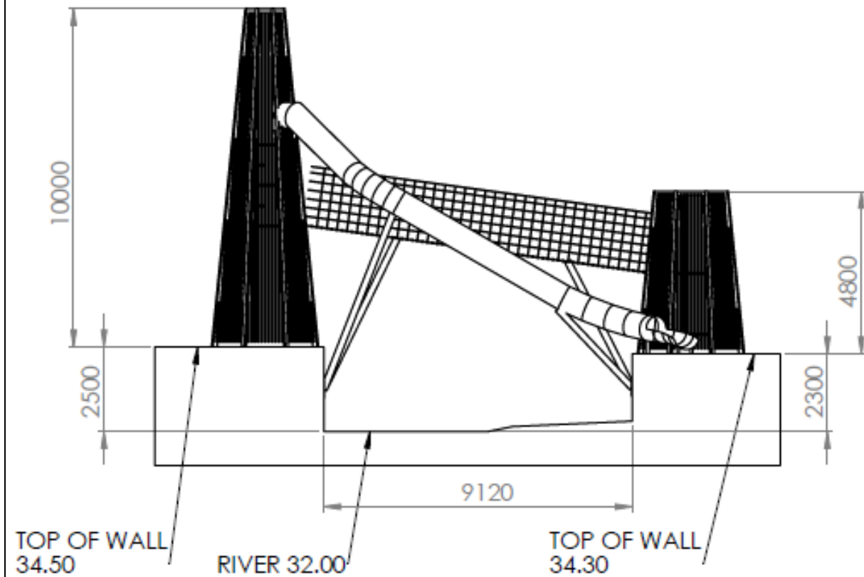
Elevation View
