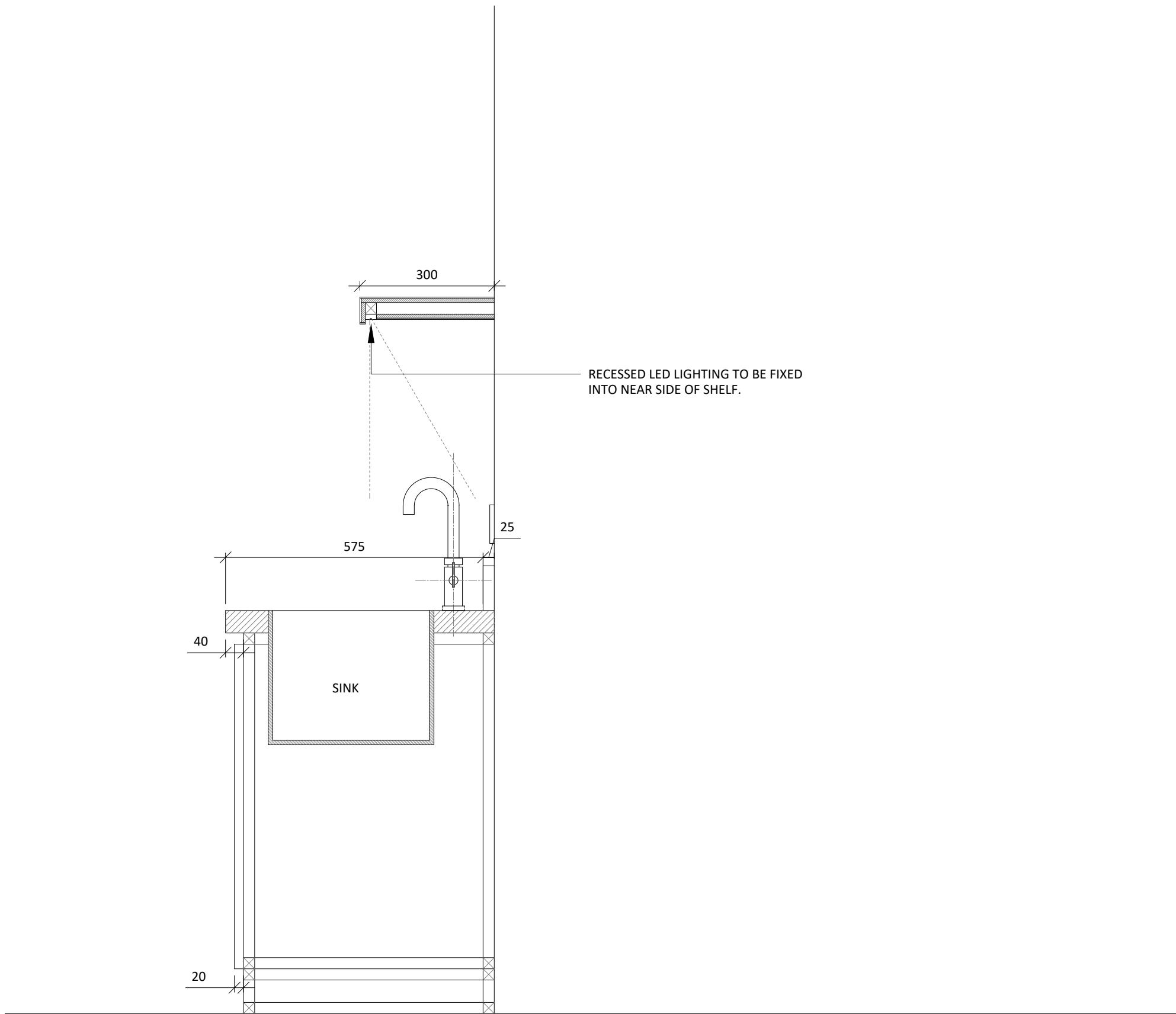
03 503 PROPOSED BANQUETTE SEATING SECTION SCALE - 1:10 @ A1 DETAILED SECTION
