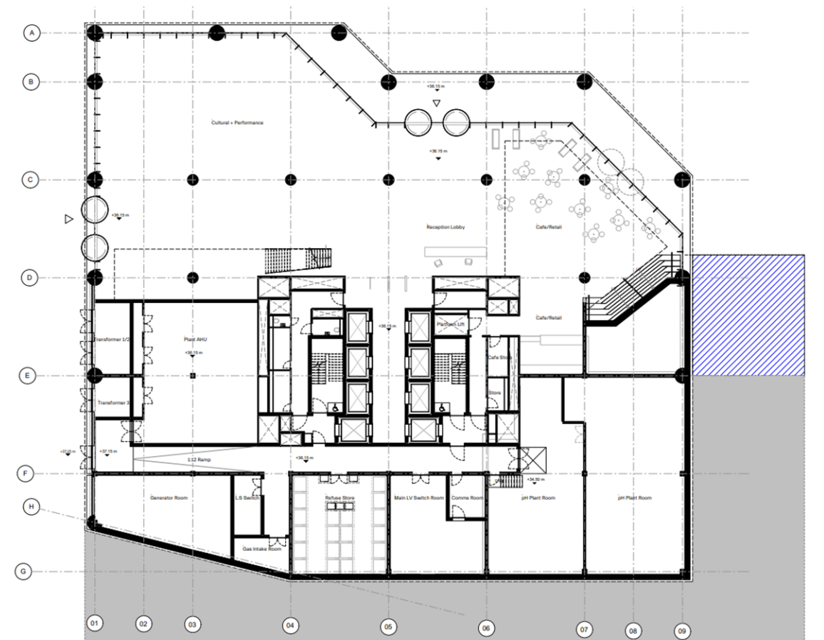
Figure 2.2 approved ground floor plan versus proposed ground floor plan
