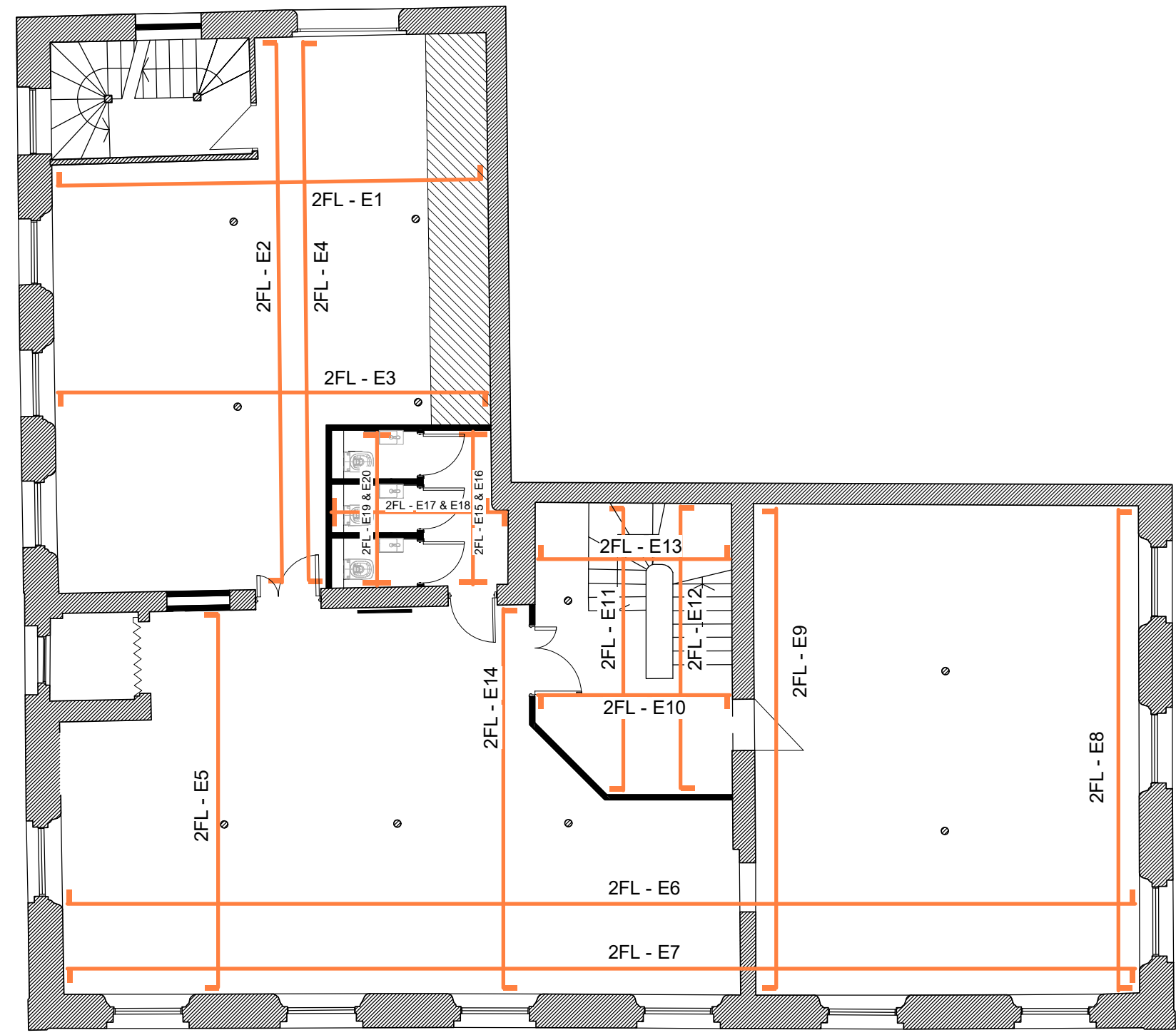
2FL Proposed Internal Elevation Layout_01
