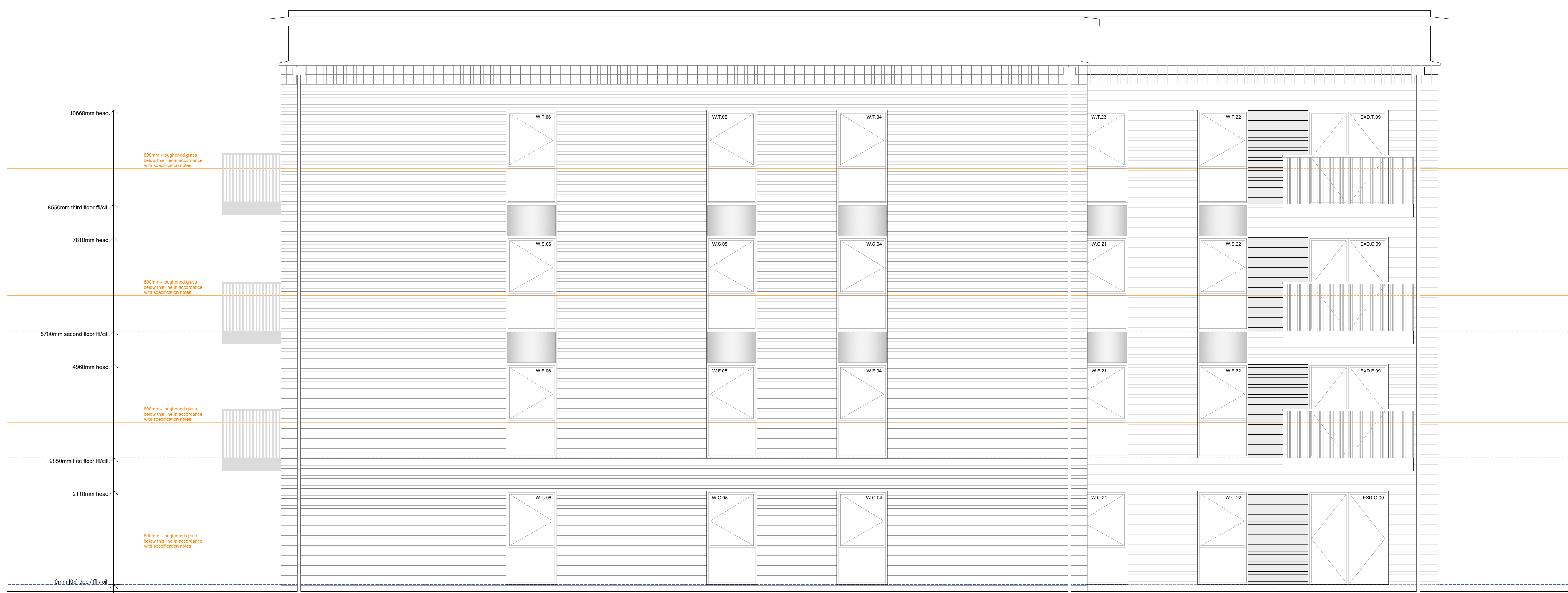
SIDE ELEVATION
