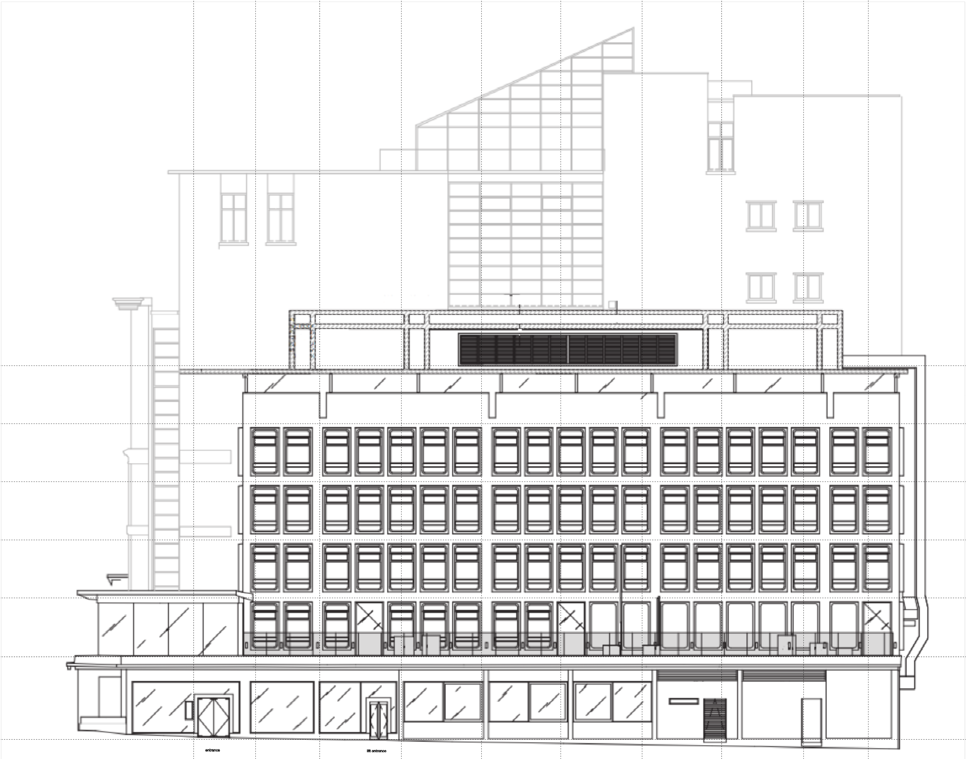
Ridgefield elevation as existing
