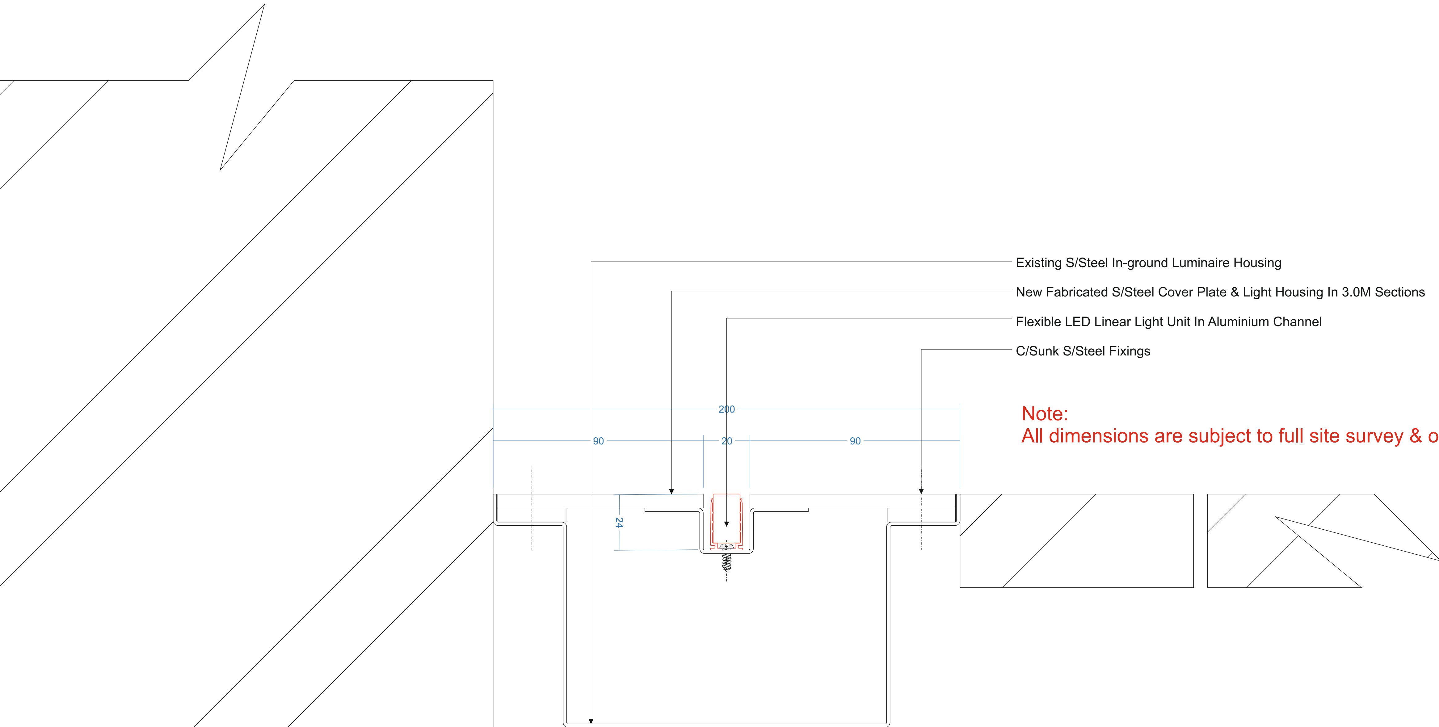
Typical Section Scale 1:10 @ A0
