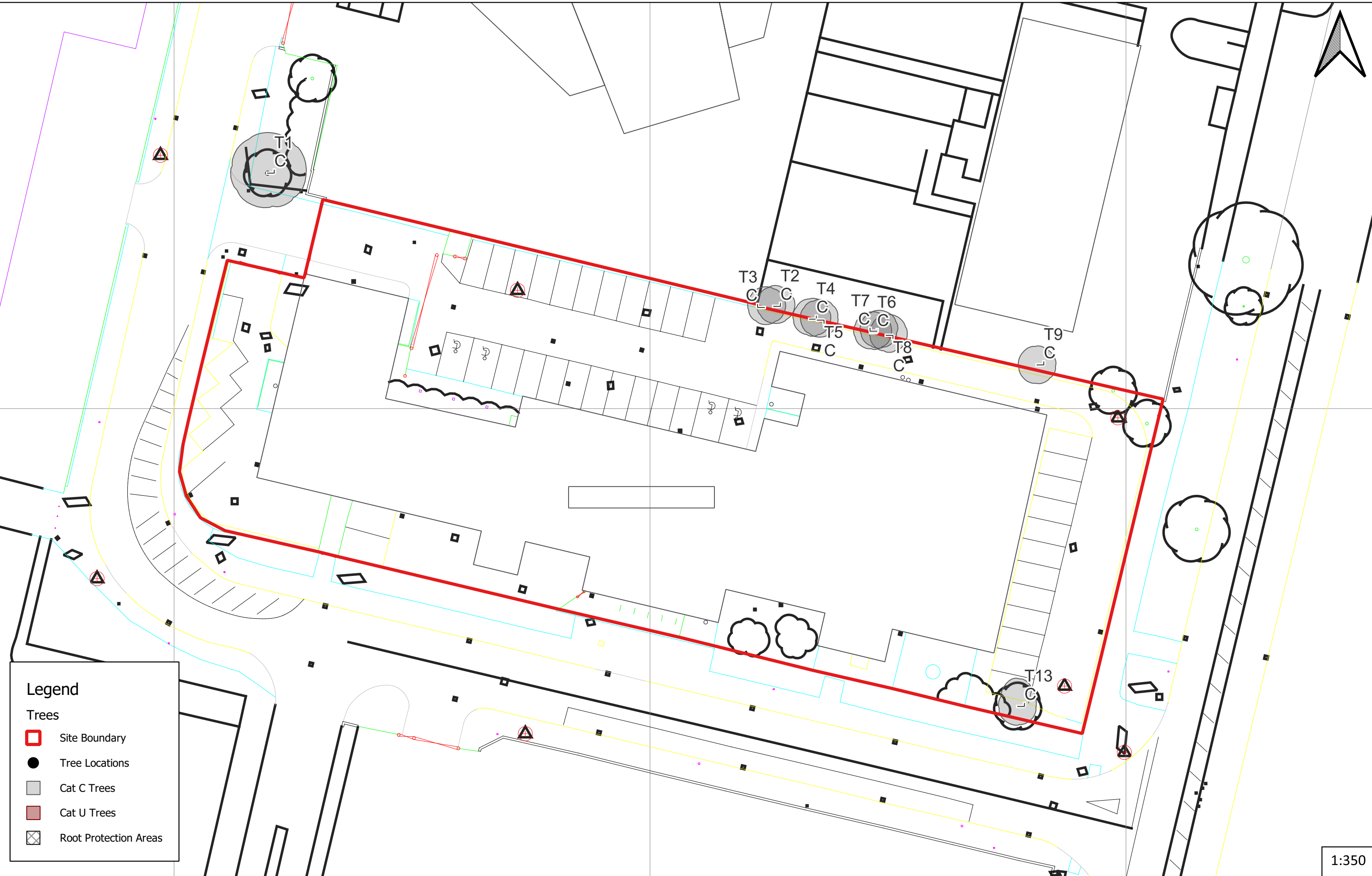
Simon House - Tree Retention Plan
