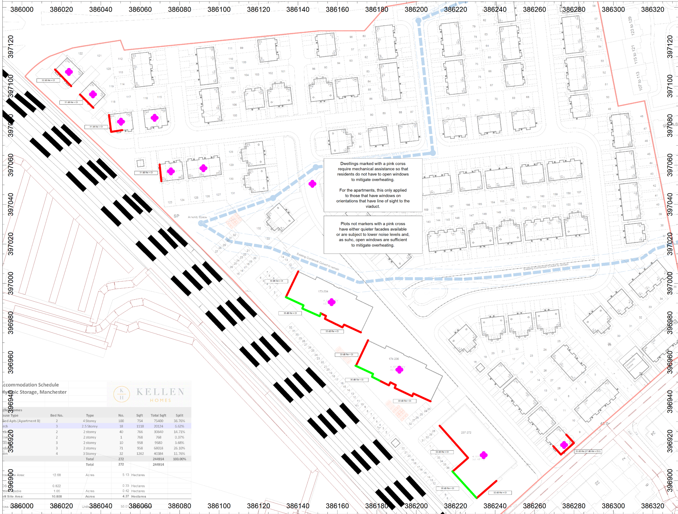
Figure 5 - Facade Insulation Requirements
