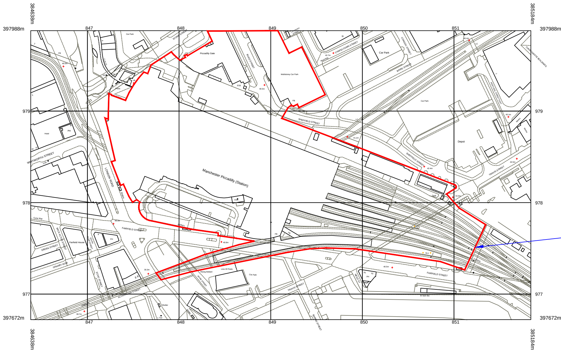
MANCHESTER PICCADILLY STATION LOCATION PLAN SCALE 1:2500
