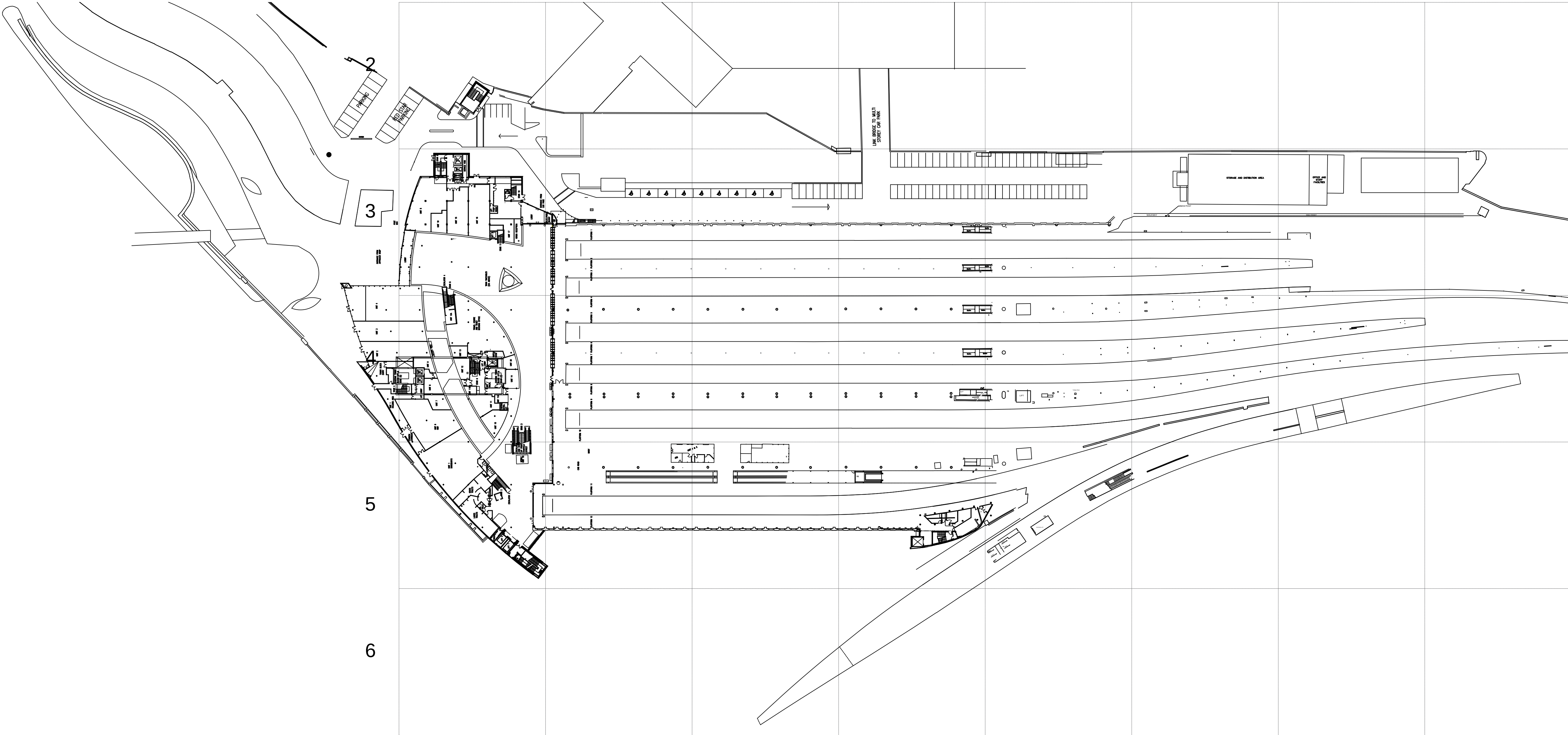
MANCHESTER PICCADILLY STATION PLAN SCALE 1:1250
