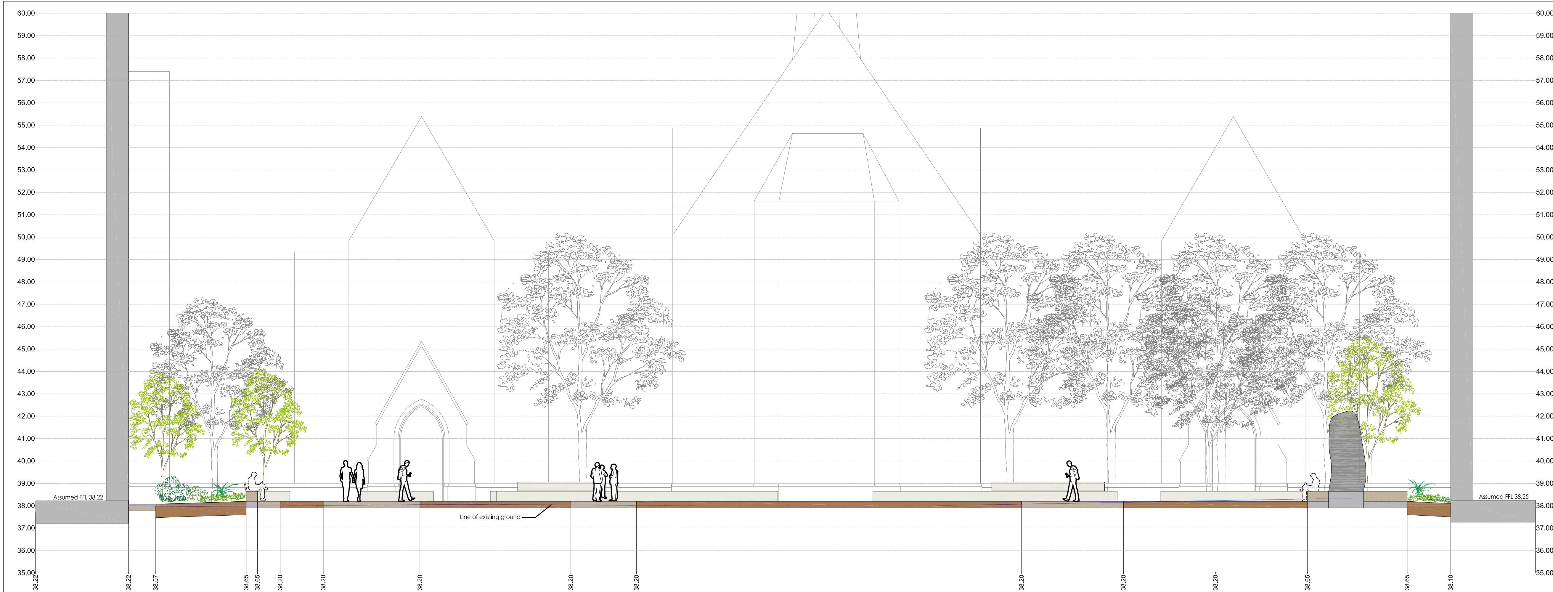
SECTION ELEVATION 1 - Scale 1:100
