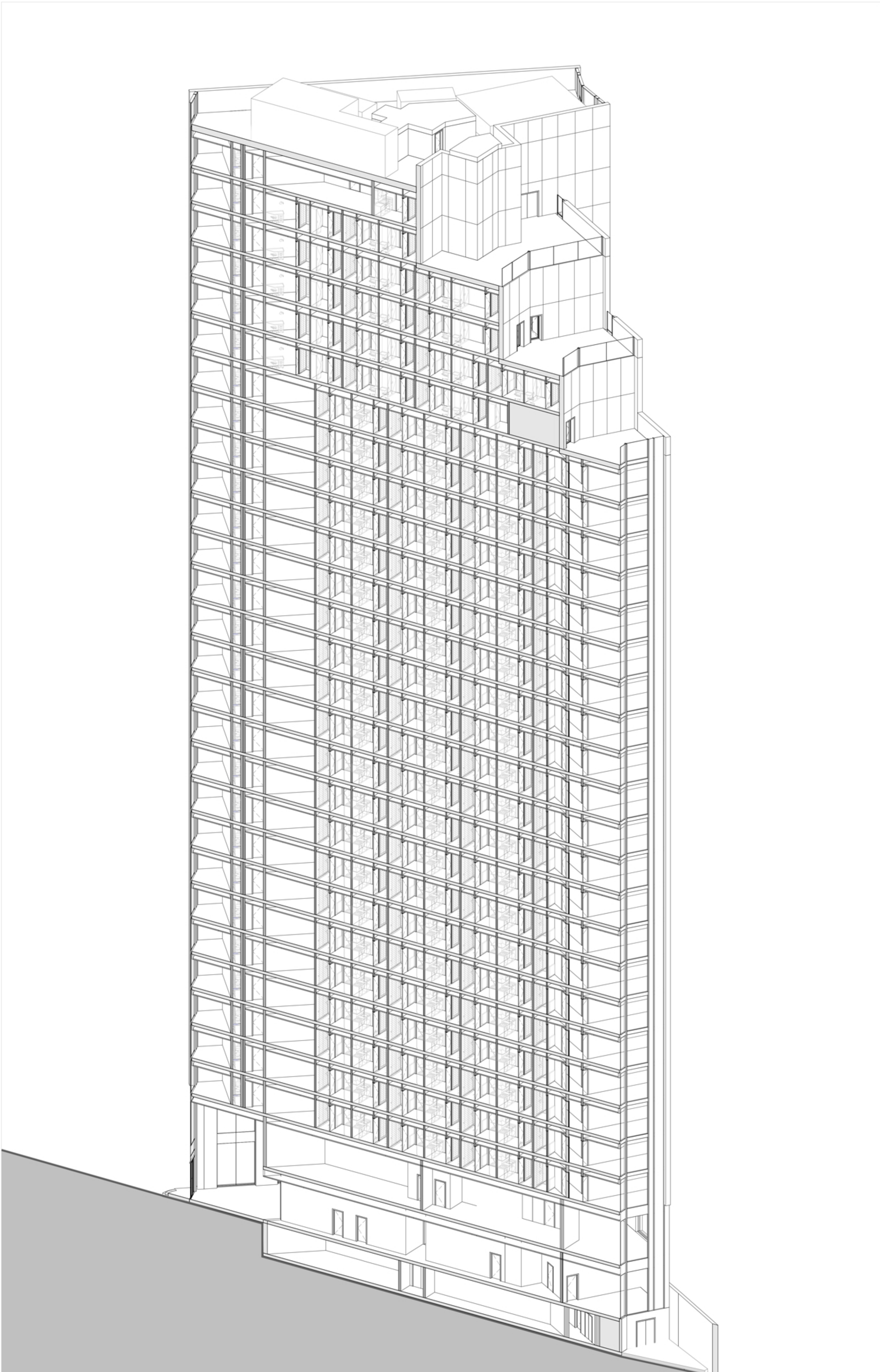
02 1:200 - 3D Isometric Section - A-A
