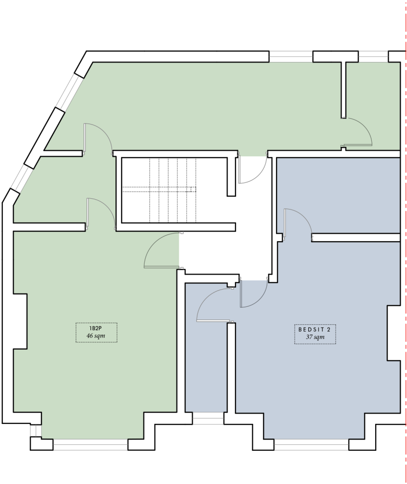
EXISTING FIRST FLOOR 1:100 @ A3
