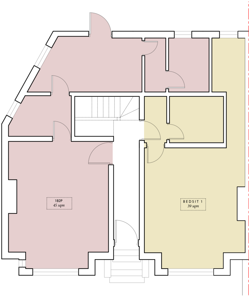
EXISTING GROUND FLOOR 1:100 @ A3 0m 1m 3m 5m
