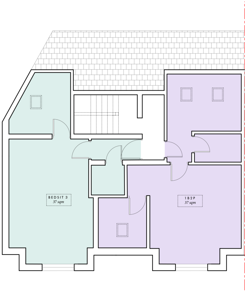
EXISTING SECOND FLOOR 1:100 @ A3
