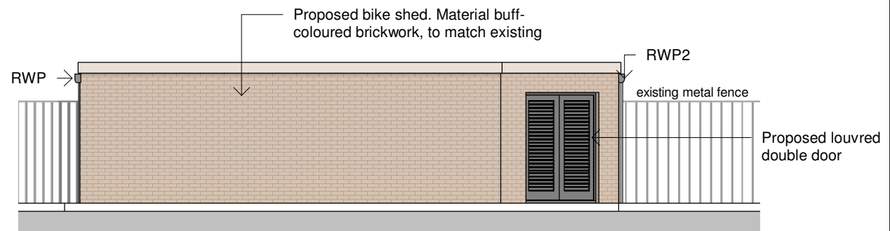
3 Proposed South Elevation 1 : 100
