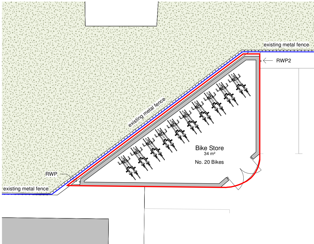
1 Proposed Floor Plan 1 : 100
