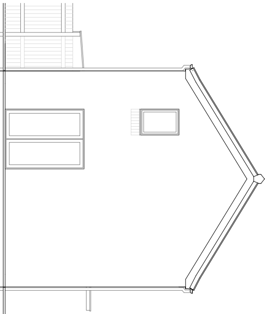
GABLE ELEVATION (EXISTING) (GARDEN SIDE)
