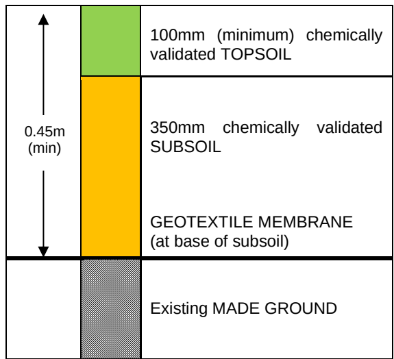
Plate 6-1: Typical Environmental Cover System Construction.
