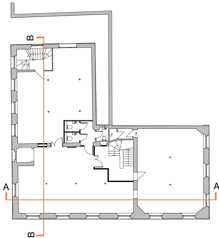
Proposed Sections Layout_00 1 : 200
