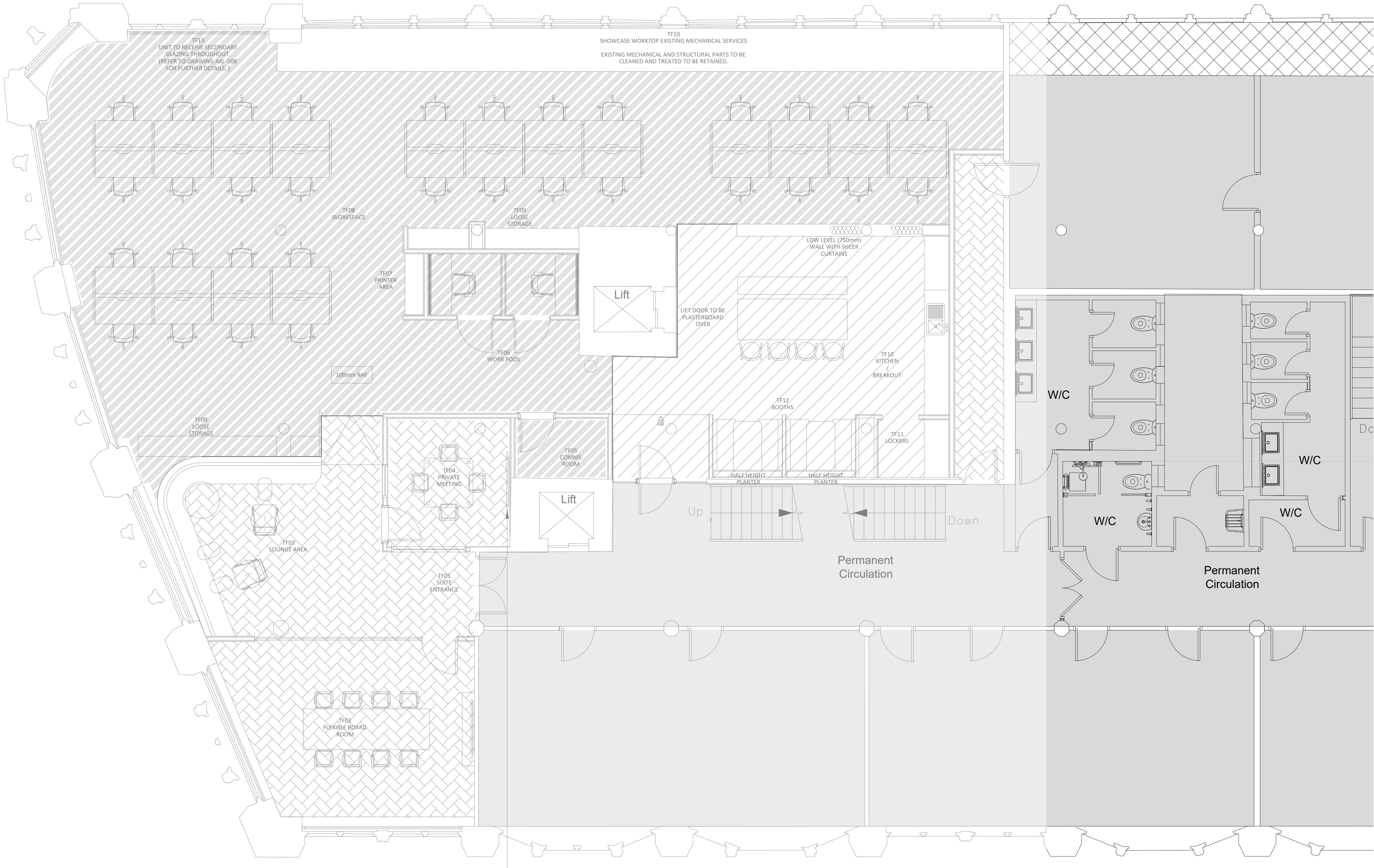
01 601 PROPOSED THIRD FLOOR SUITE FLOOR FINISHES PLAN SCALE - 1:50 @ A1 AS PROPOSED
