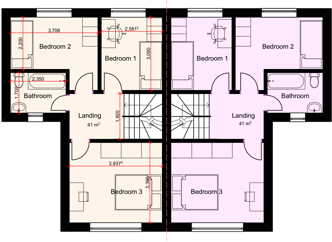
PROPOSED GA FIRST FLOOR PLAN UNITS 1- 4
