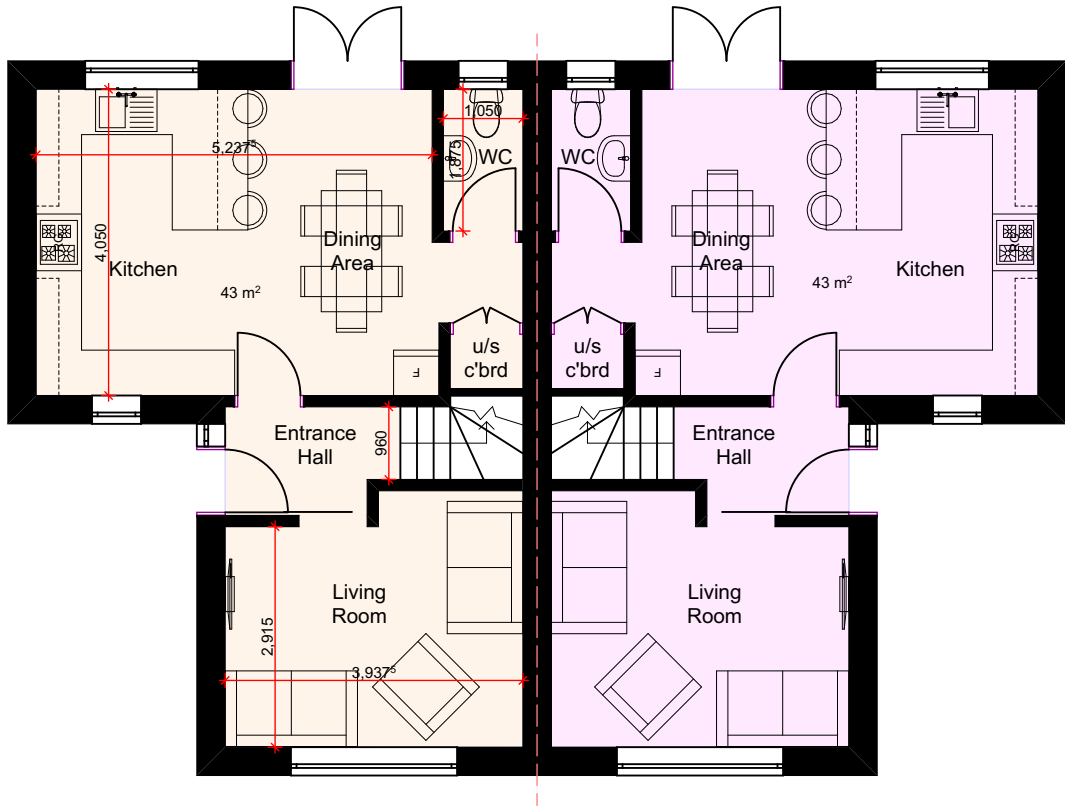
PROPOSED GA GROUND FLOOR PLAN UNITS 1- 4
