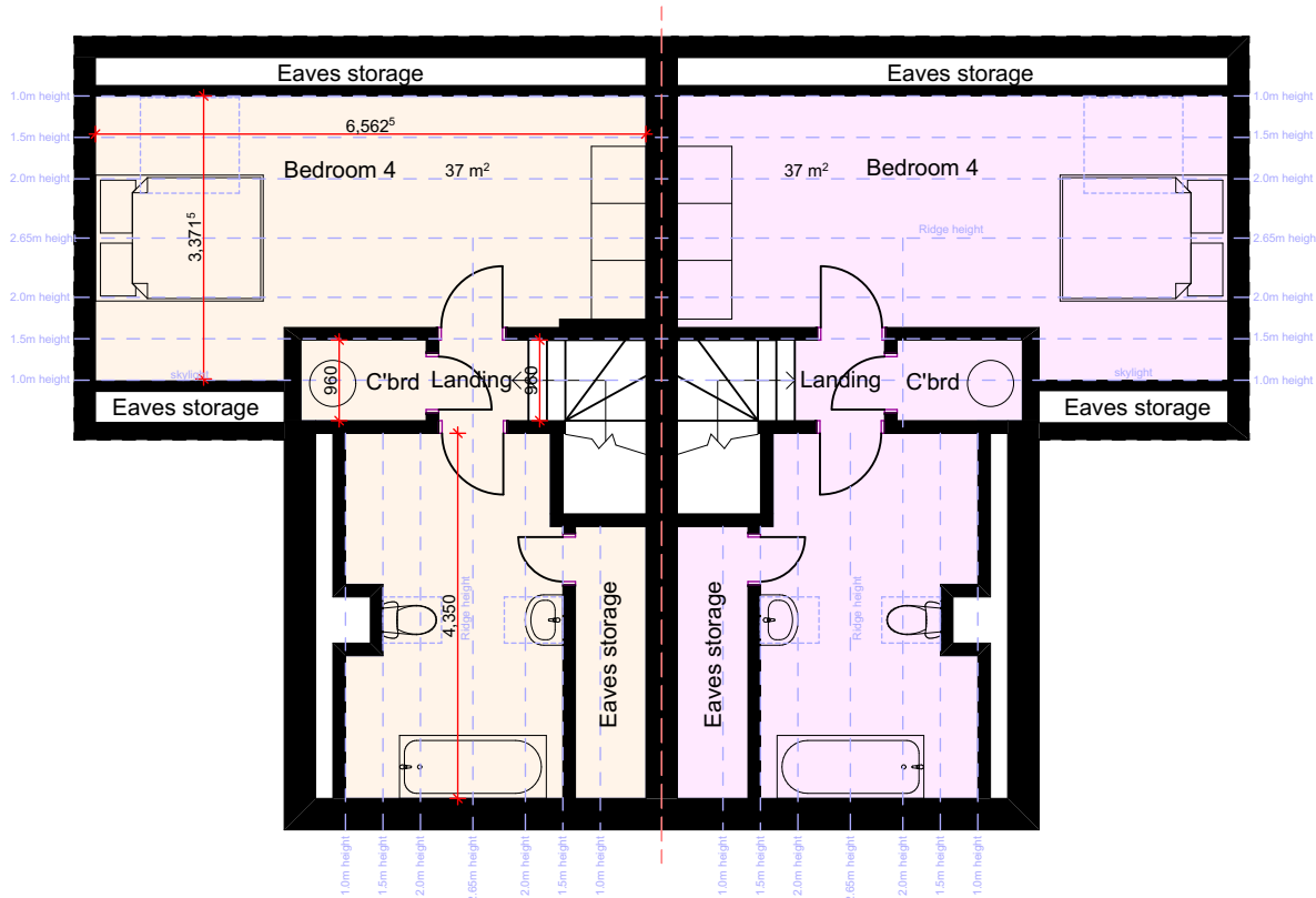
PROPOSED GA SECOND FLOOR PLAN UNITS 1- 4
