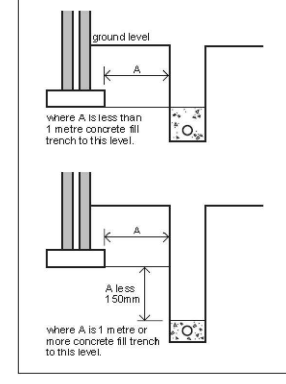
Diagram 8: Pipe runs near buildings
