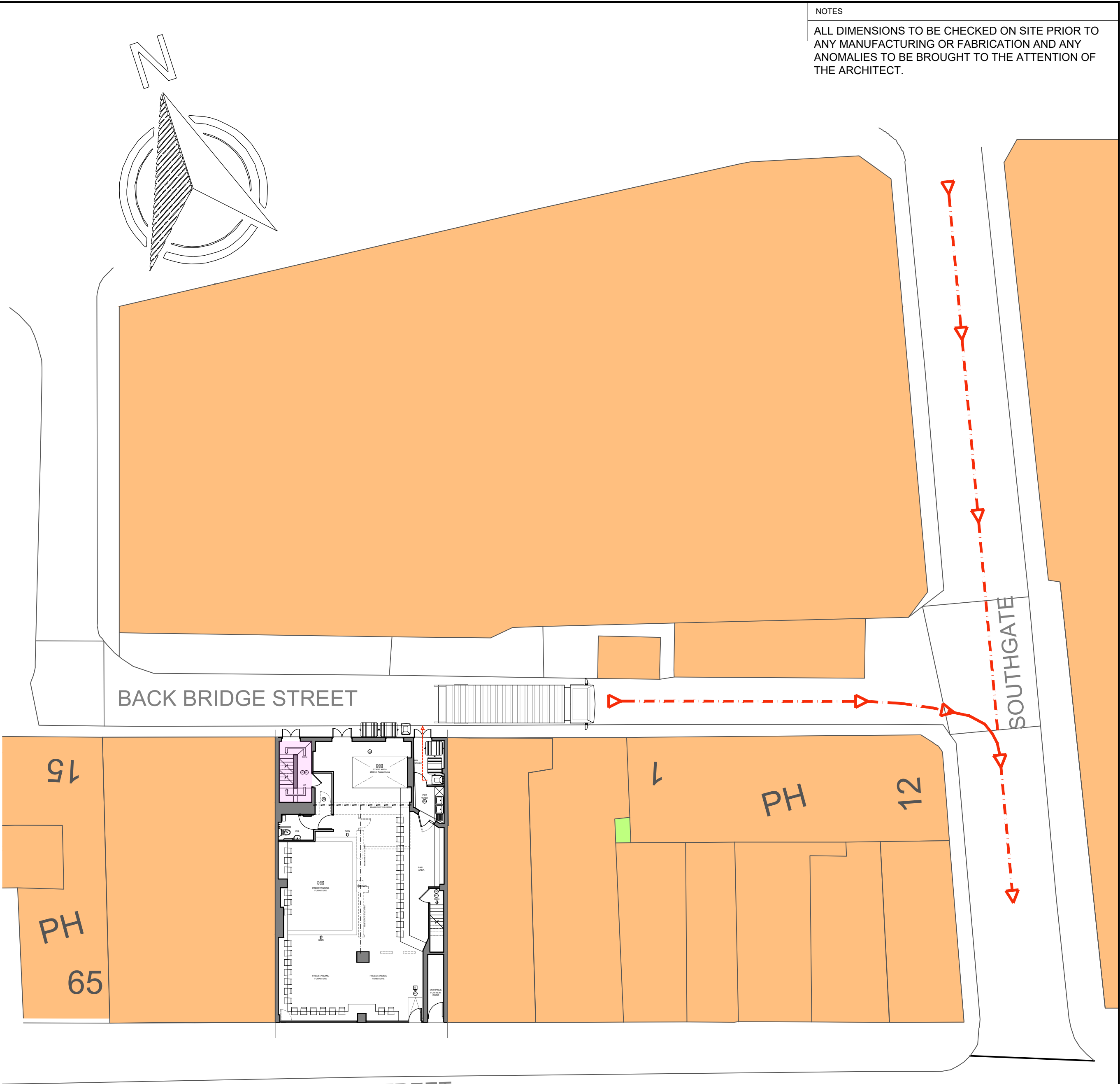
REFUSE VEHICLE MOVEMENT PLAN 1:200
