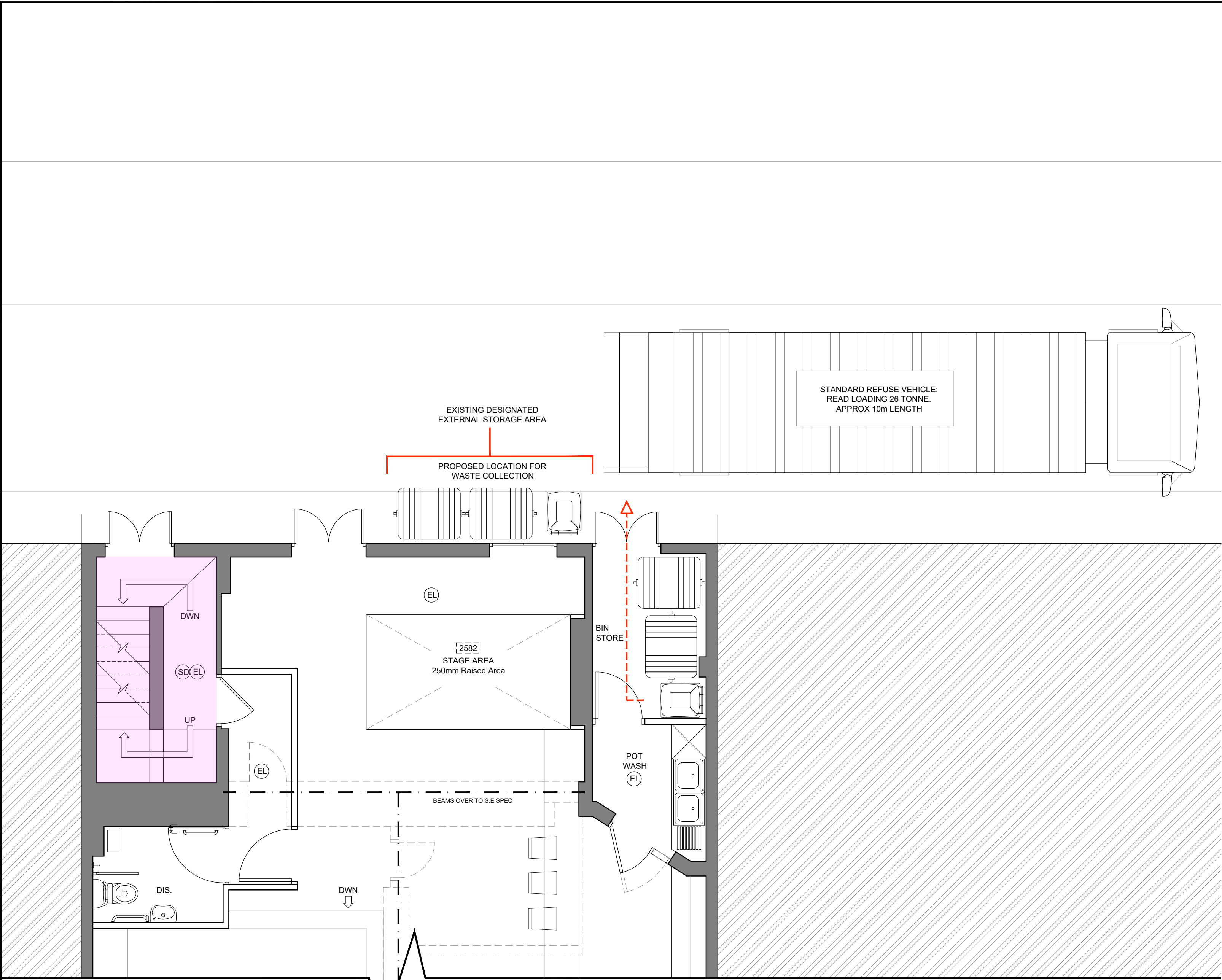
REFUSE PICKUP PLAN 1:50
