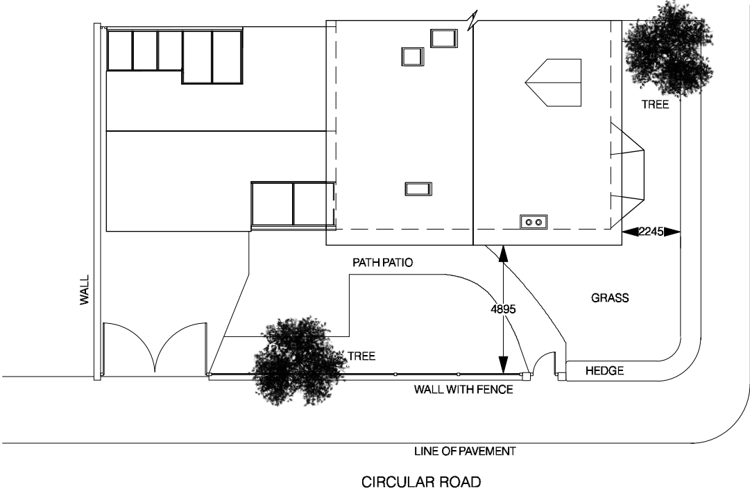
SITE PLAN PROPOSED
