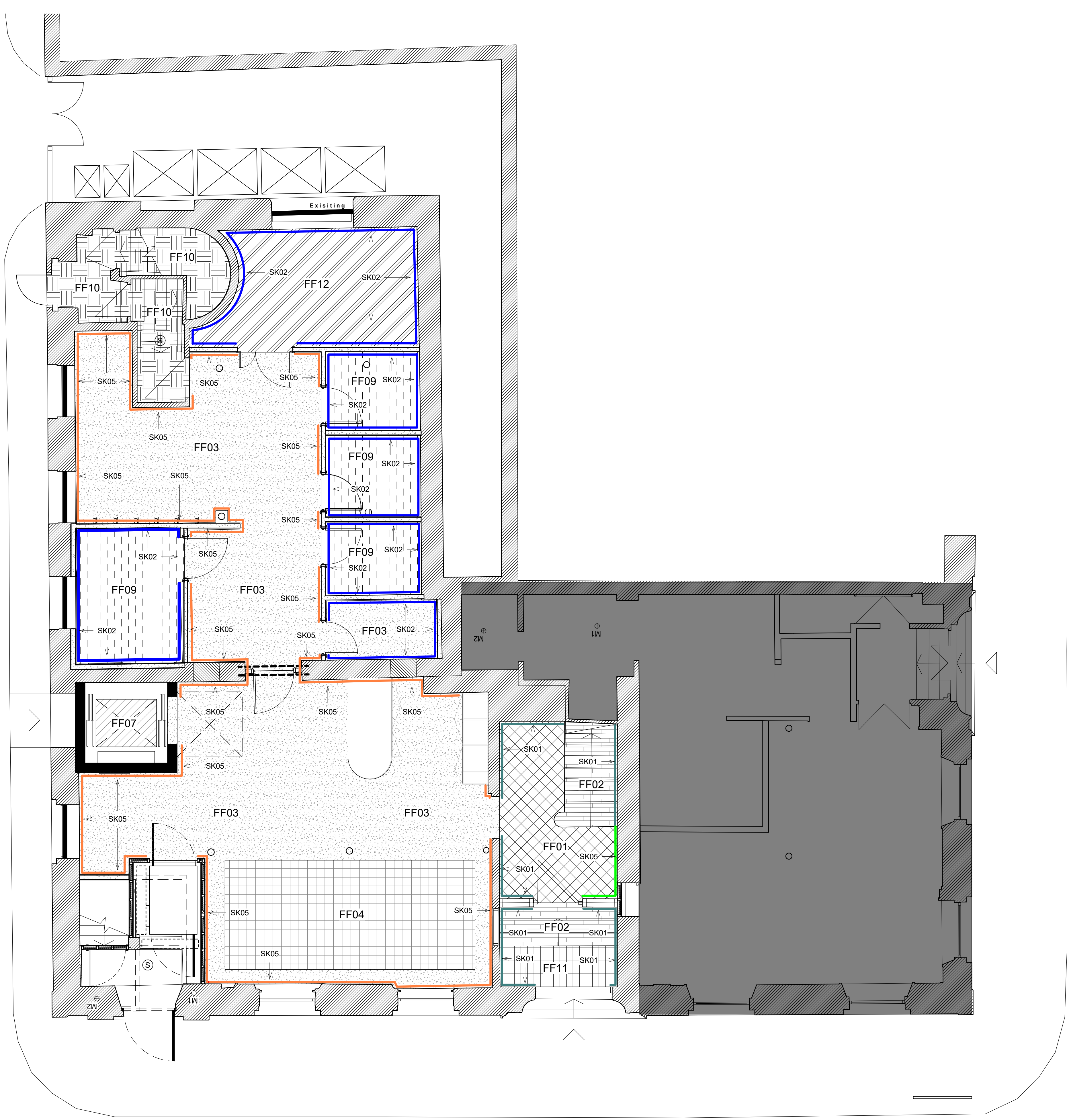
GFL Proposed Floor Finishes 1 : 50
