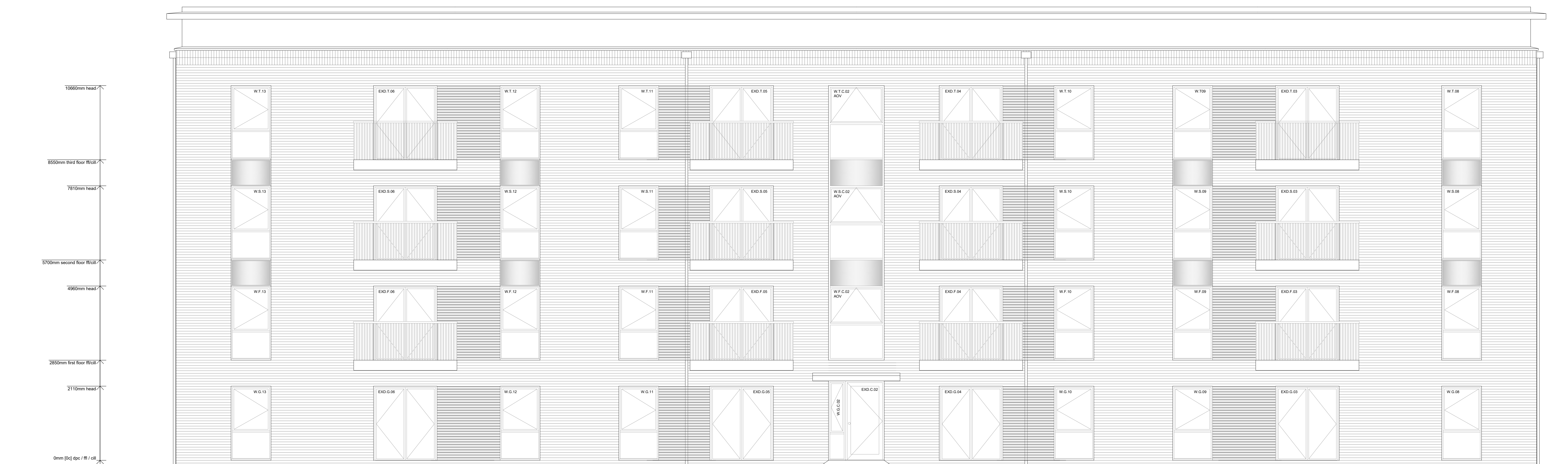
REAR ELEVATION
