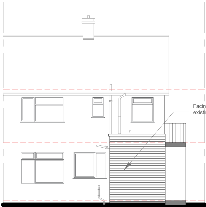
Rear Elevation
