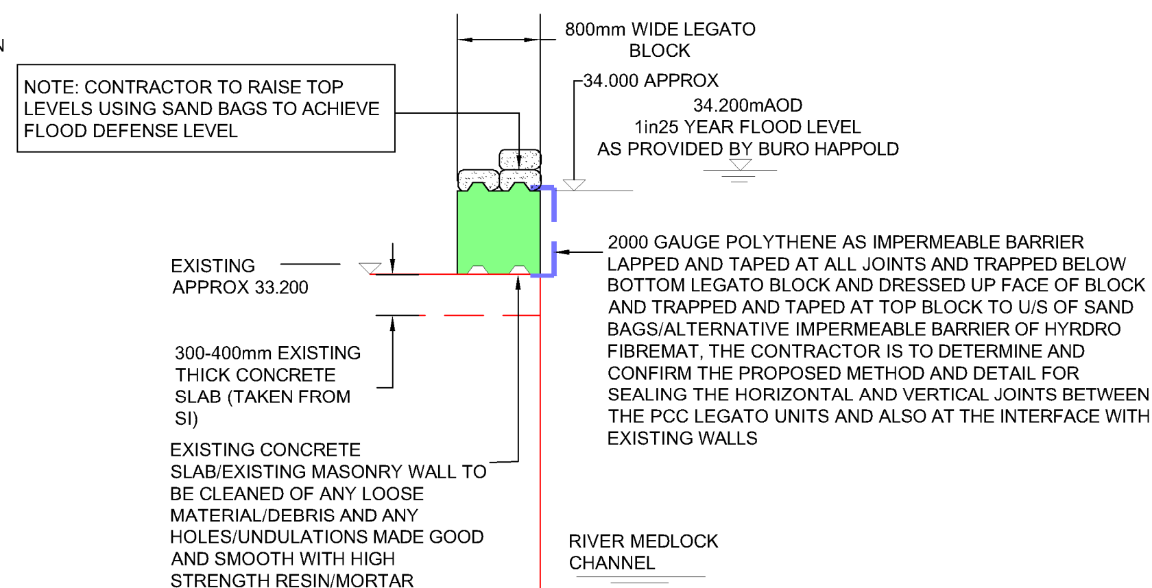
SECTION THROUGH WALL AT APPROX CHAINAGE 20 ON ELEVATION 1
