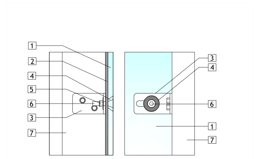
FASTENING GLASS DETAIL
