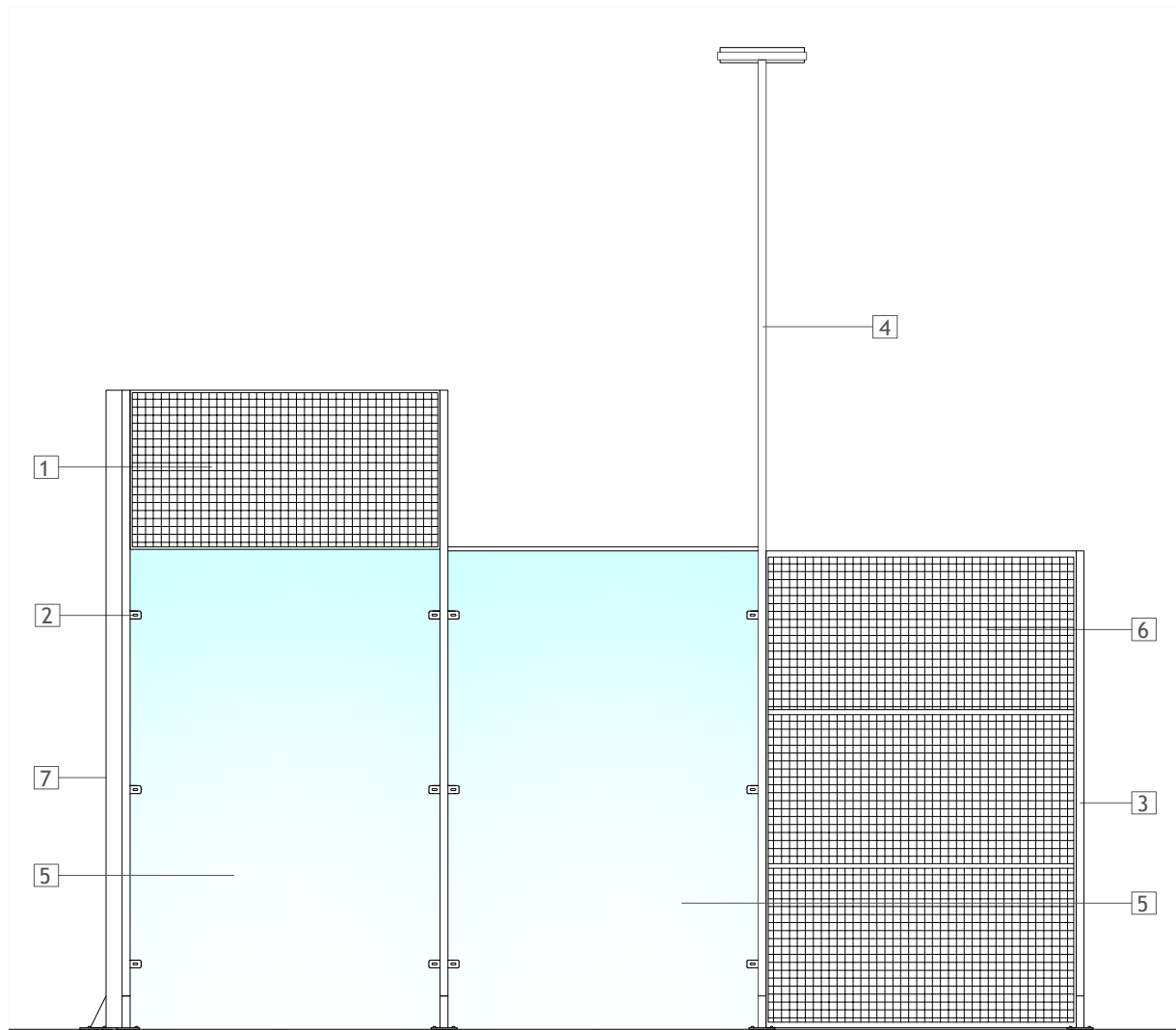
DETAIL OF LATERAL VIEW
