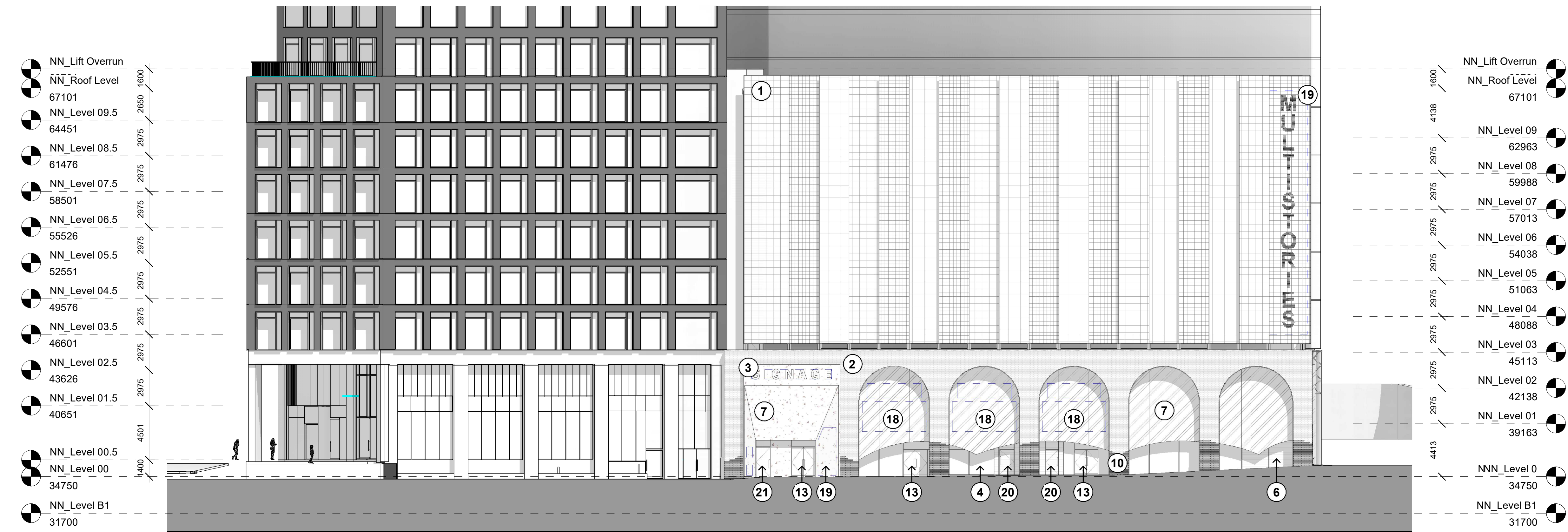
2 Proposed - Elevation - West (Contextual) 1 : 200
