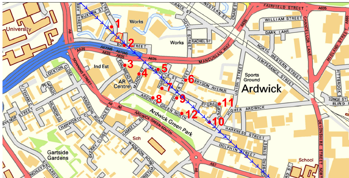
Figure 8 - Surveyed Locations. The blue arrows indicate the direction of the incoming DTT signals from Winter Hill transmitter
