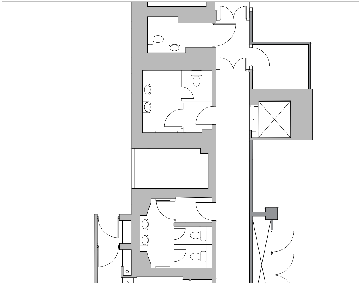
Level 03 WC - 1:100
